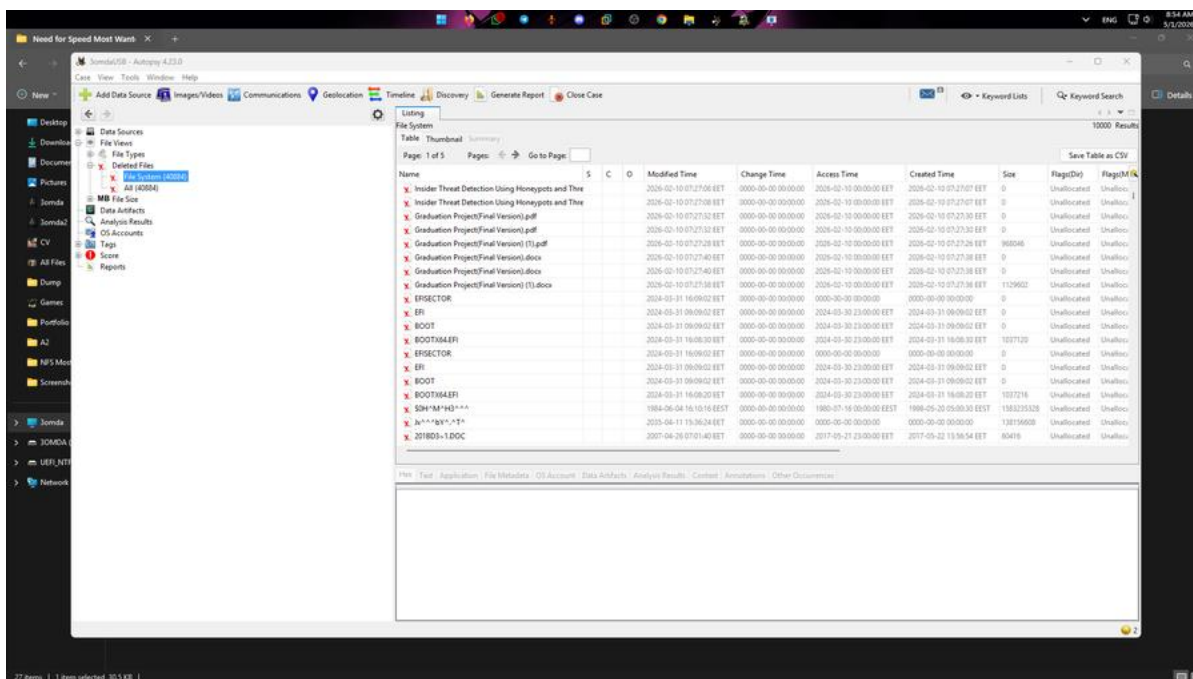
Figure 13: Deleted Files — File System View Showing 40,884 Unallocated Entries with Key Artifacts
