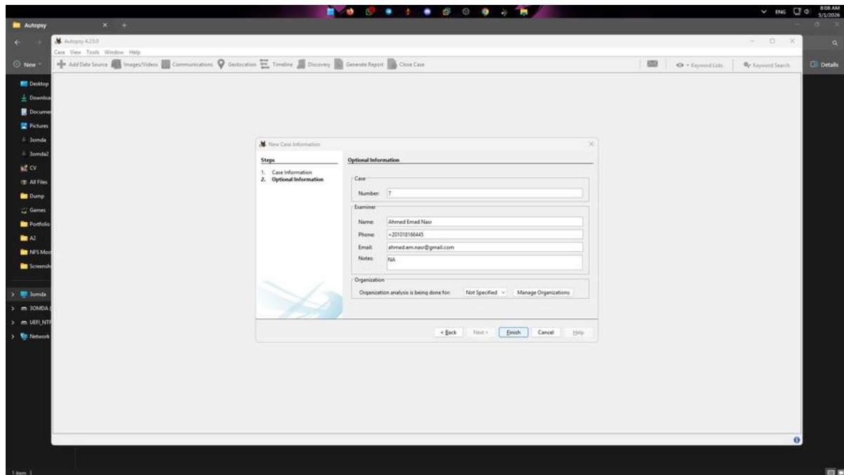
Figure 3: New Case Optional Information — Examiner Metadata Entry
