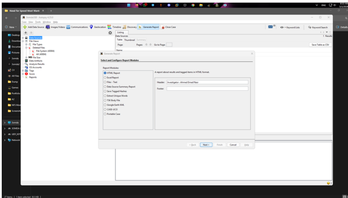
Figure 12: Generate Report Dialog — HTML Report Selected with Custom Investigator Header
