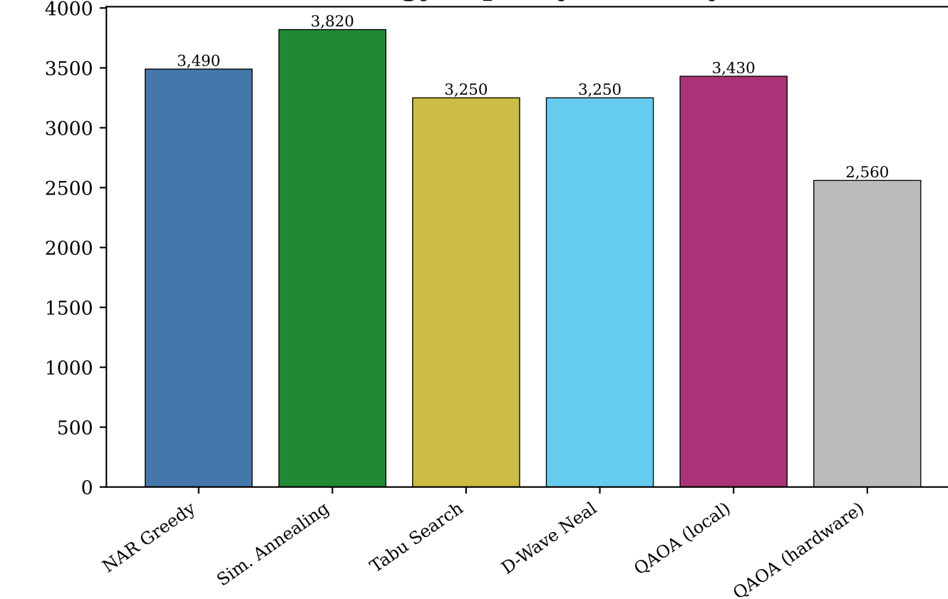
Energy Capacity (kWh/day)
