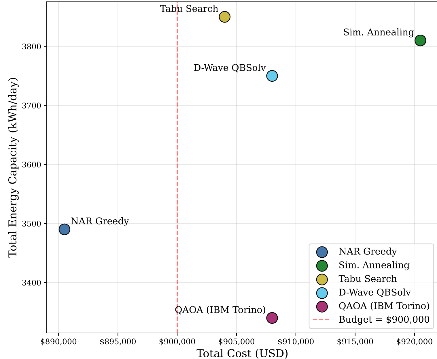
Cost vs Energy Capacity
