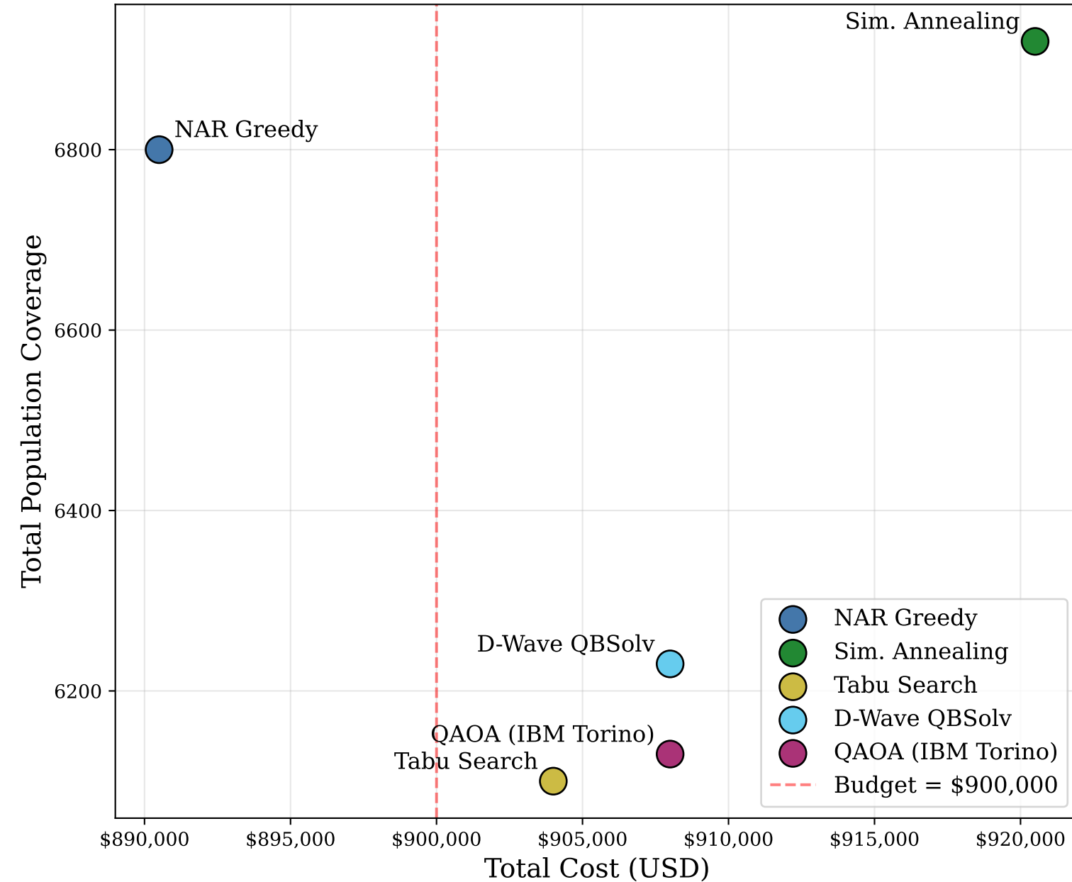
Cost vs Population Coverage
