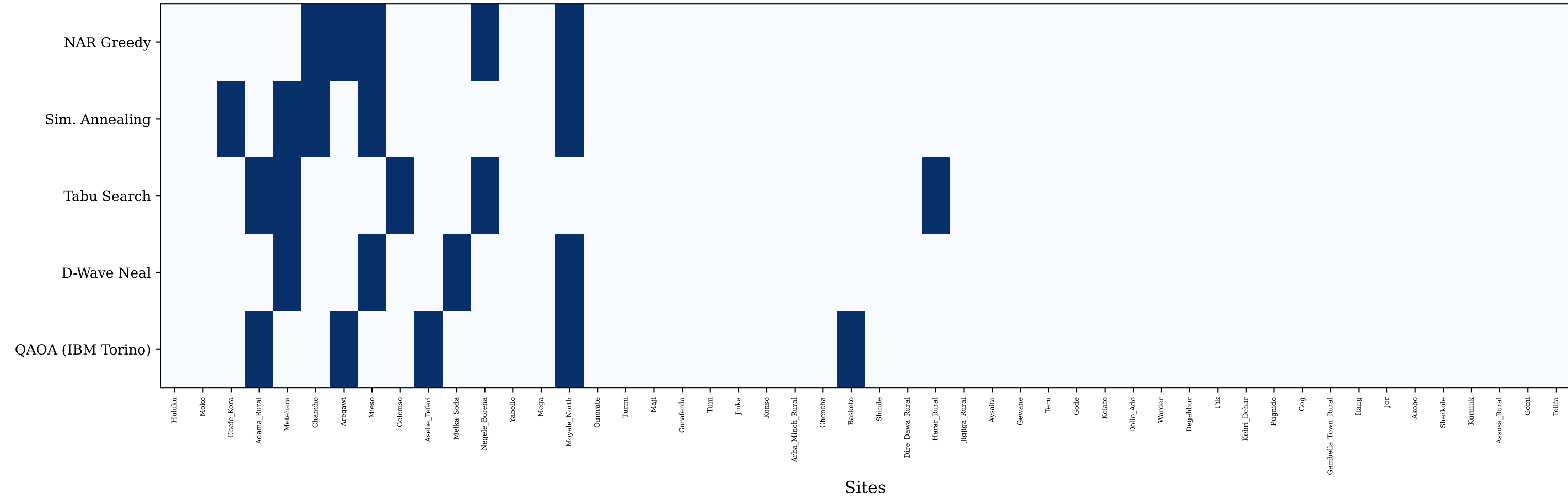
Solution Matrix (blue = selected)
