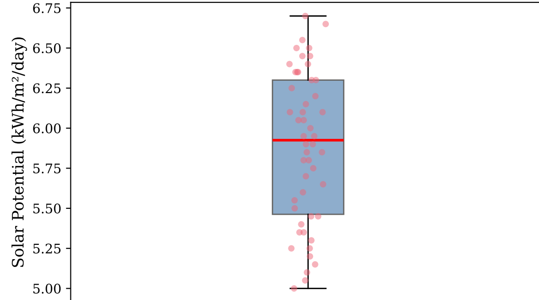
Distribution of Solar Potential (kWh/m 2 /day)
