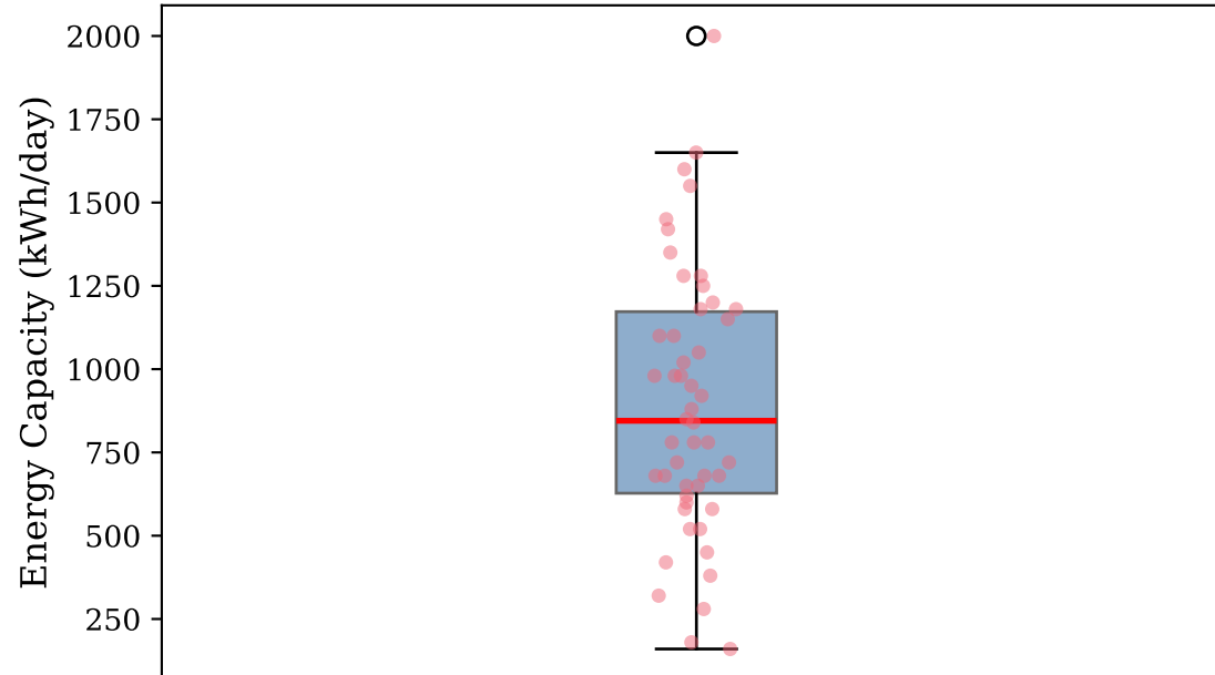
Distribution of Energy Capacity (kWh/day)
