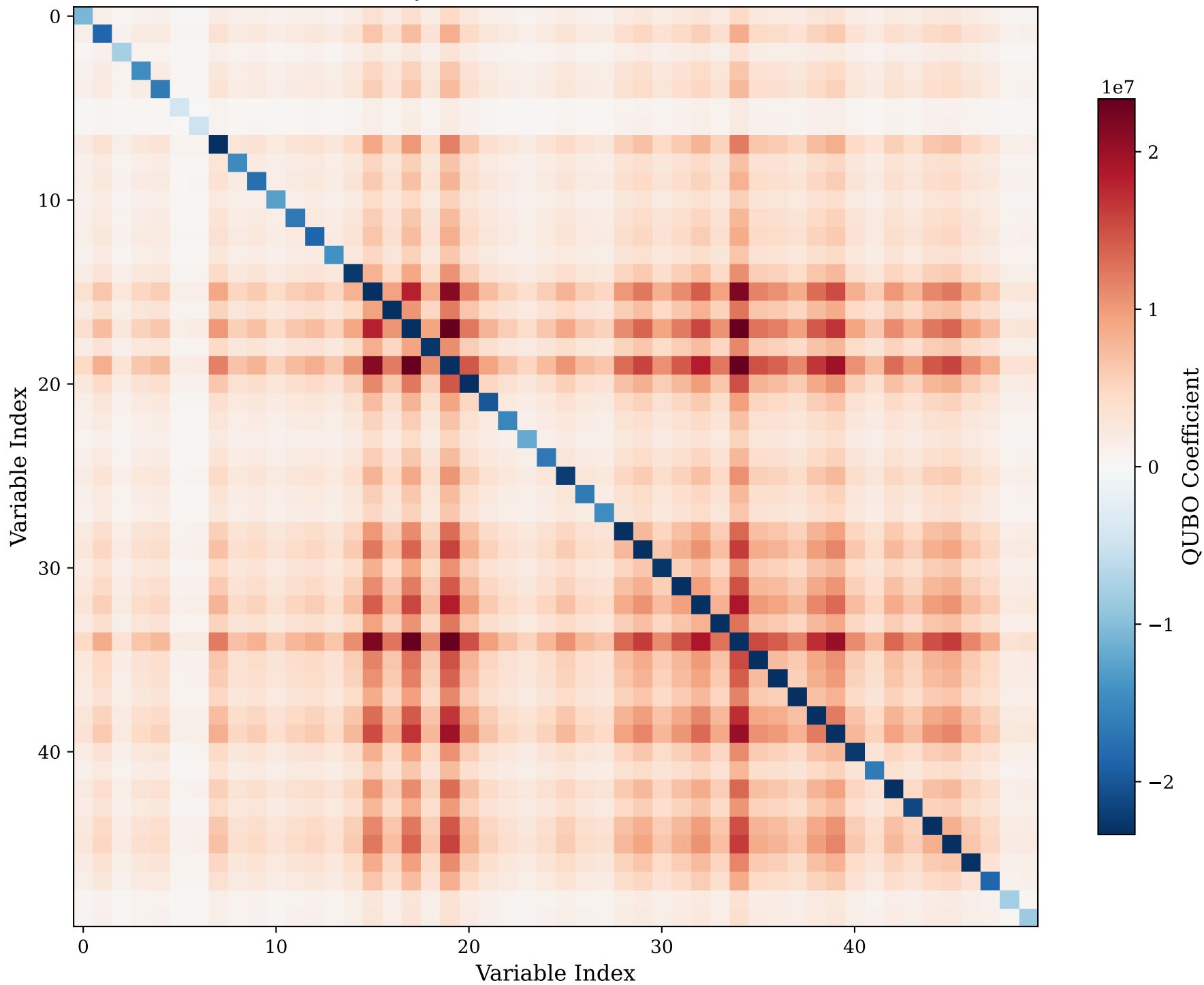
QUBO Matrix (50x50)
