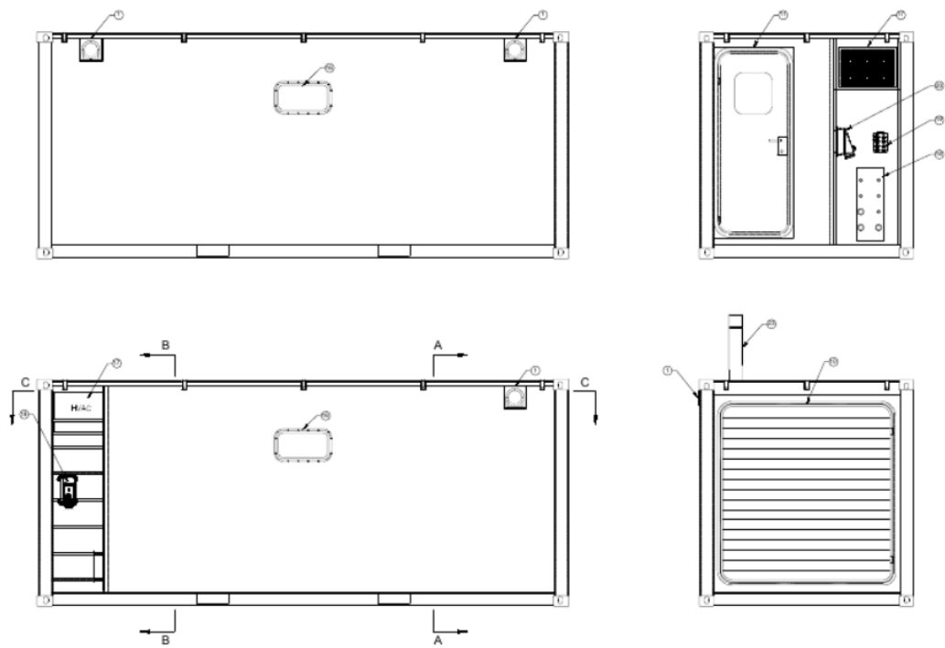
EXTERNAL SIDE AND END VIEWS SCALE 1:15
