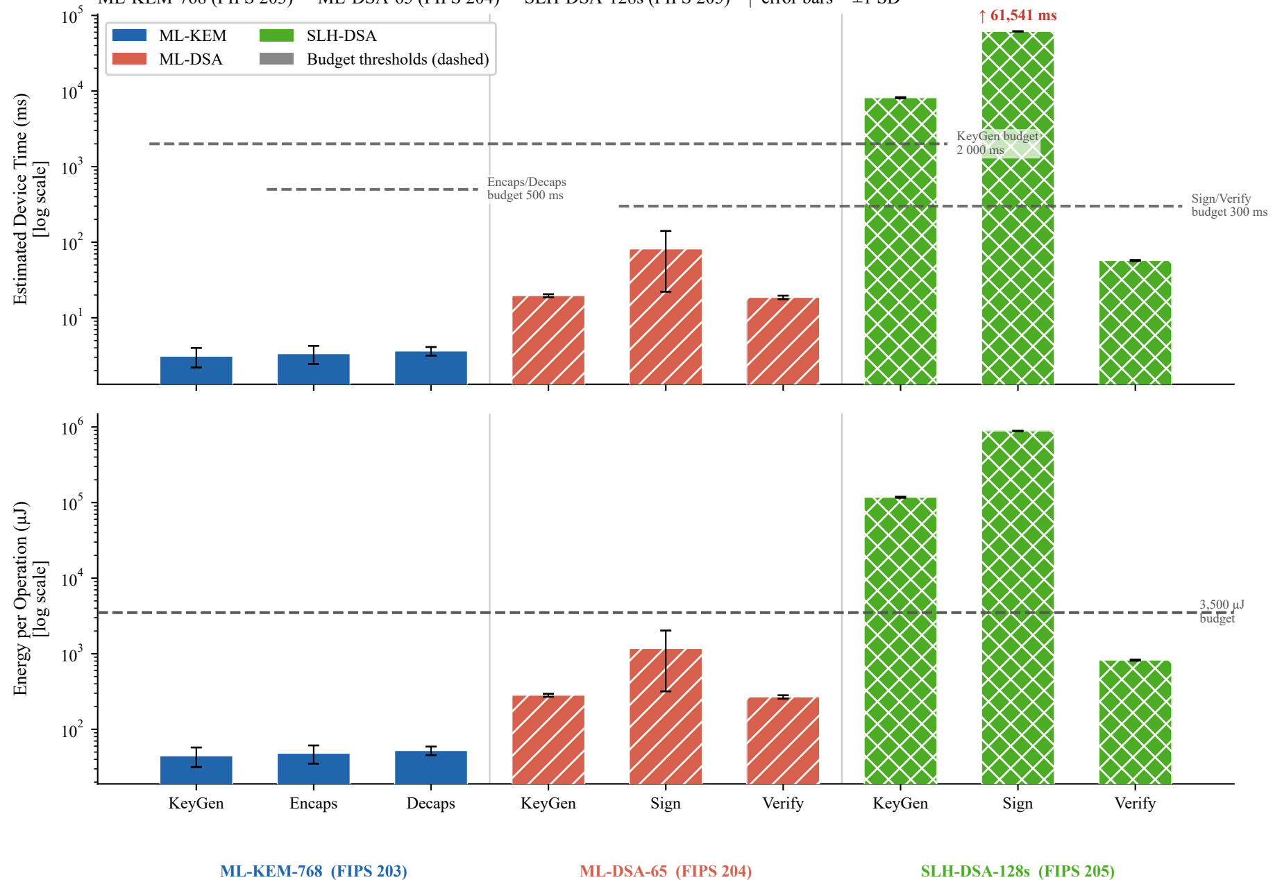
Fig. A Cryptographic Operation Performance on Nordic nRF52840 (Cortex-M4F @ 64 MHz) ML-KEM-768 (FIPS 203) · ML-DSA-65 (FIPS 204) · SLH-DSA-128s (FIPS 205) | error bars = \pm 1 SD
