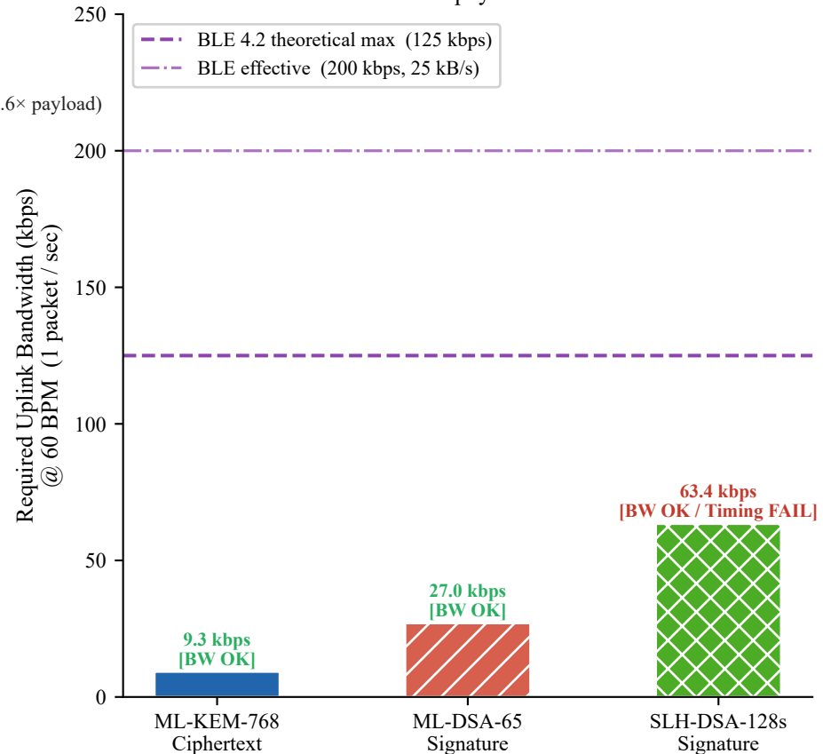
(b) Required uplink bandwidth vs BLE 4.2 physical limits
