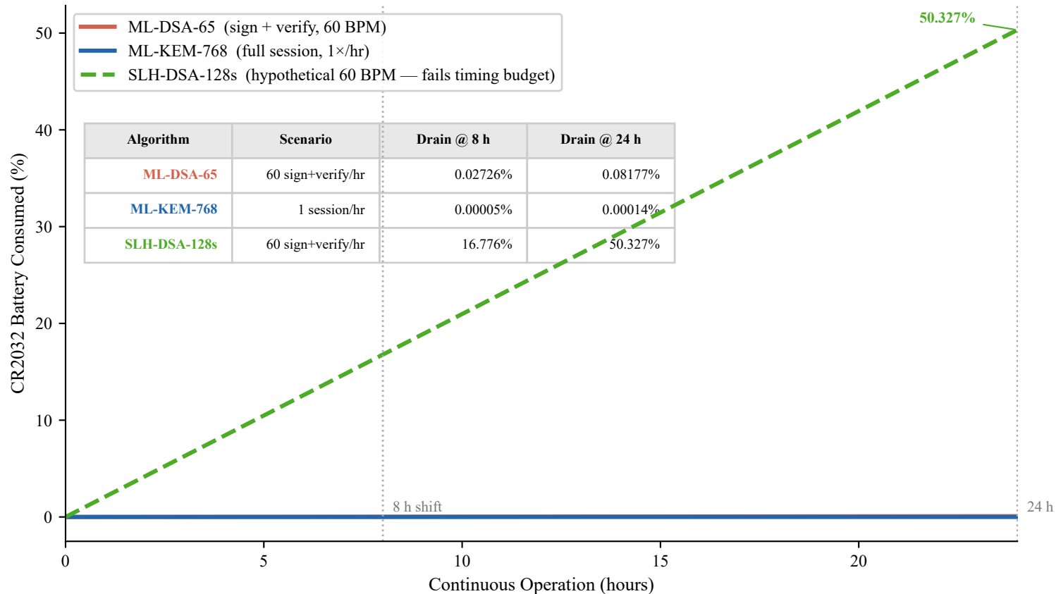
Fig. D Cumulative CR2032 Battery Drain — 24-Hour Clinical Operation CR2032 = 2.54 J · Active power model: 14.4 mW · HR = 60 BPM
