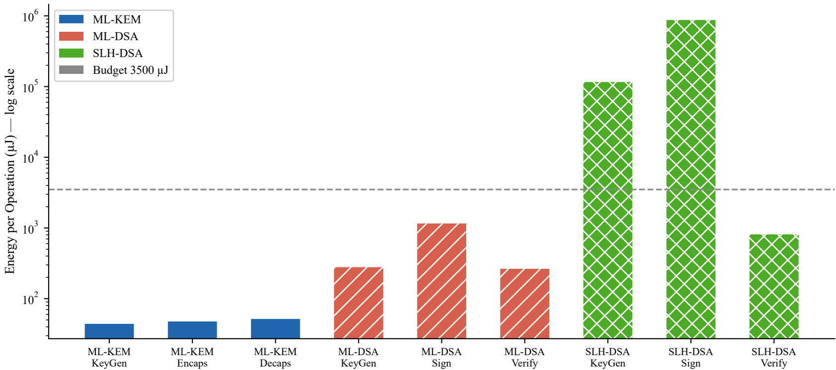
Fig. 2 Energy Consumption per Cryptographic Operation CR2032 @ 3 V · 14.4 mW active power model
