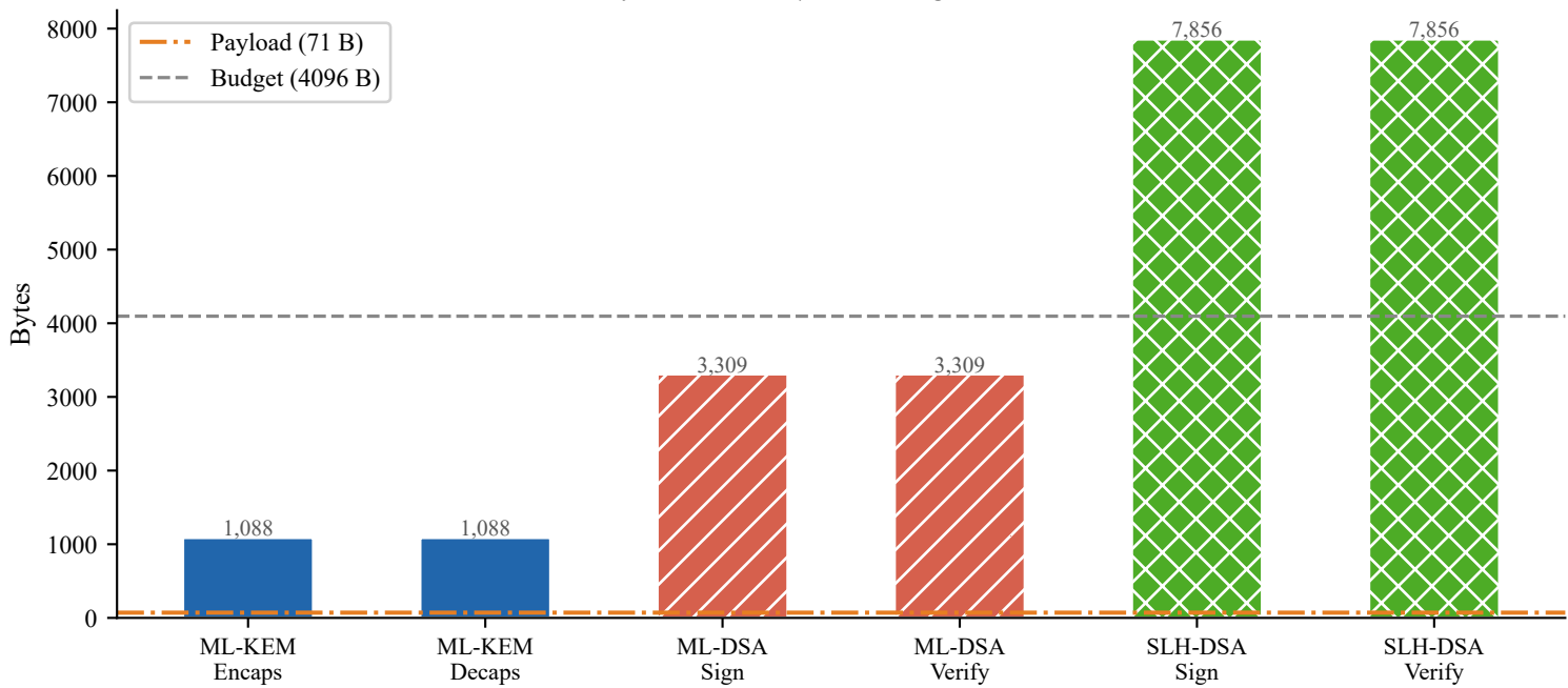
Fig. 4 Ciphertext / Signature Size vs Heartbeat Payload Payload = 71 B | BLE budget = 4096 B
