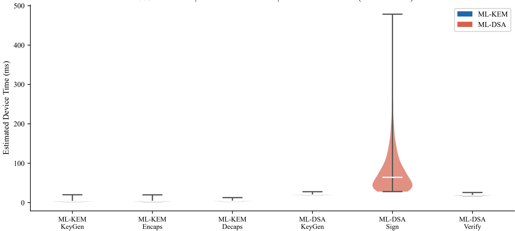
Fig. 5 Latency Distribution per Operation (ML-KEM & ML-DSA) 1 000 trials each | white line = median | SLH-DSA excluded (extreme scale)
