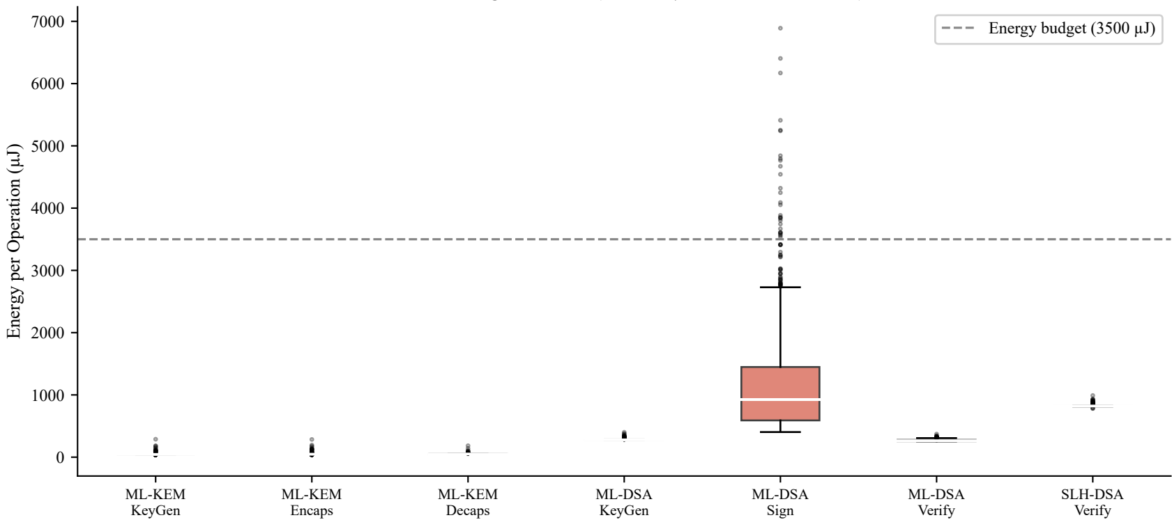
Fig. 6 Energy Distribution per Operation (Box-and-Whisker) SLH-DSA Sign excluded (883 885 \mu\text{J} median — off scale)
