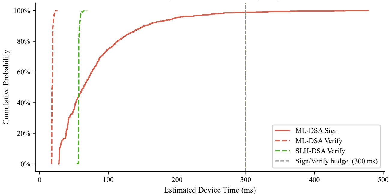
Fig. 7 Empirical CDF of Per-Packet Sign & Verify Latency All trials | dotted verticals = timing budget
