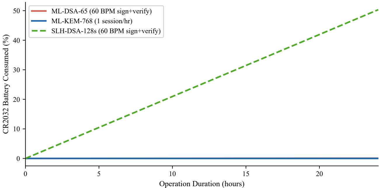
Fig. 8 Cumulative Battery Drain Projection CR2032 = 2.54 J | Active power = 14.4 mW
