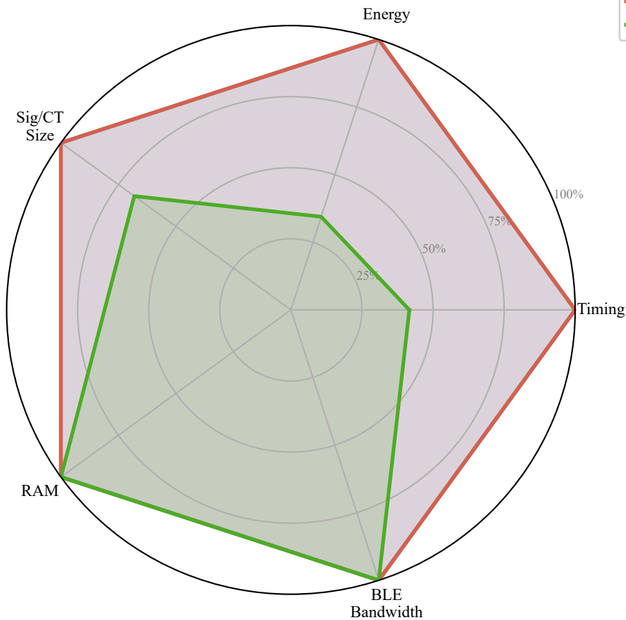
Fig. 10 Multi-Criteria Feasibility Radar
