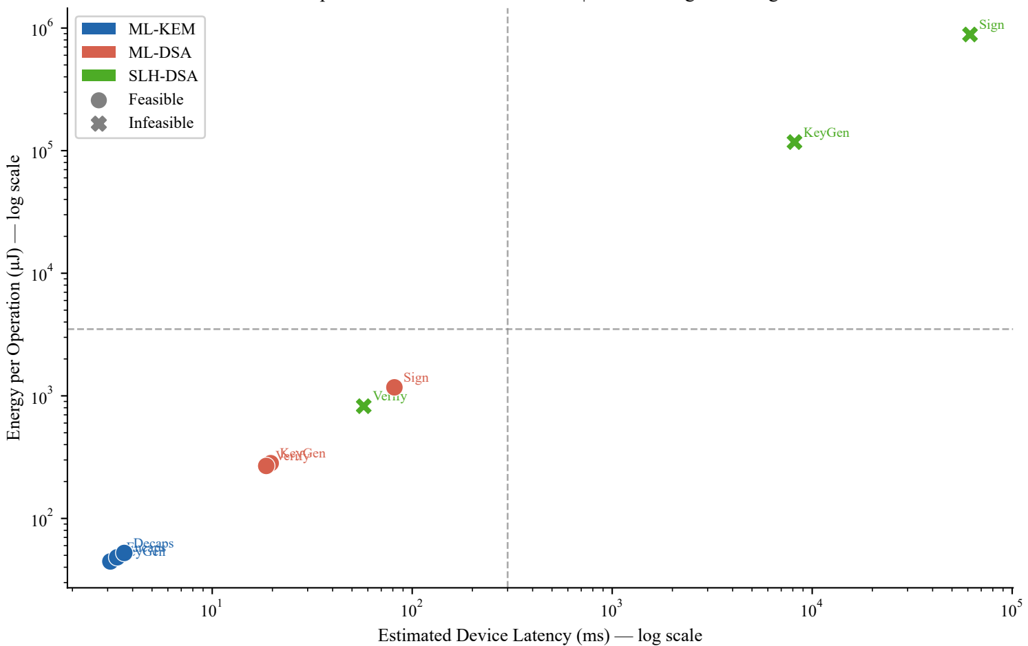
Fig. 11 Latency–Energy Tradeoff Space
