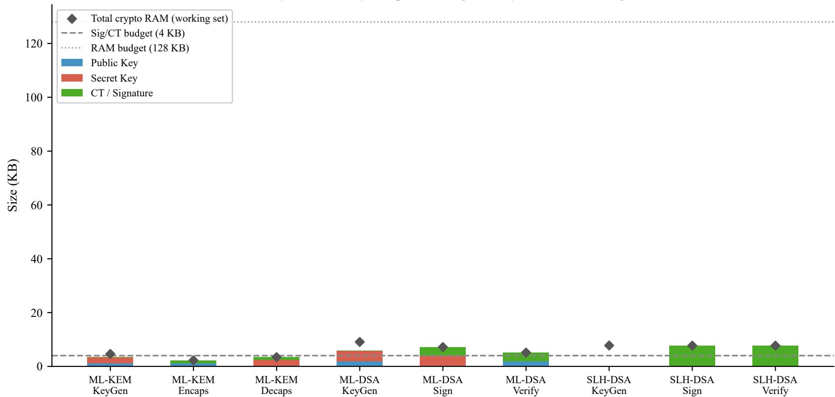
Fig. 3 Cryptographic Object Memory Footprint Public Key + Secret Key + Ciphertext/Signature | = total working RAM
