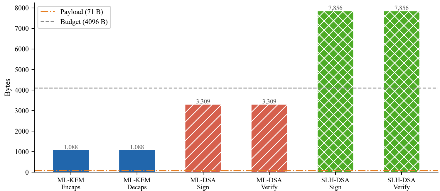
Fig. 4 Ciphertext / Signature Size vs Heartbeat Payload Payload = 71 B | BLE budget = 4096 B
