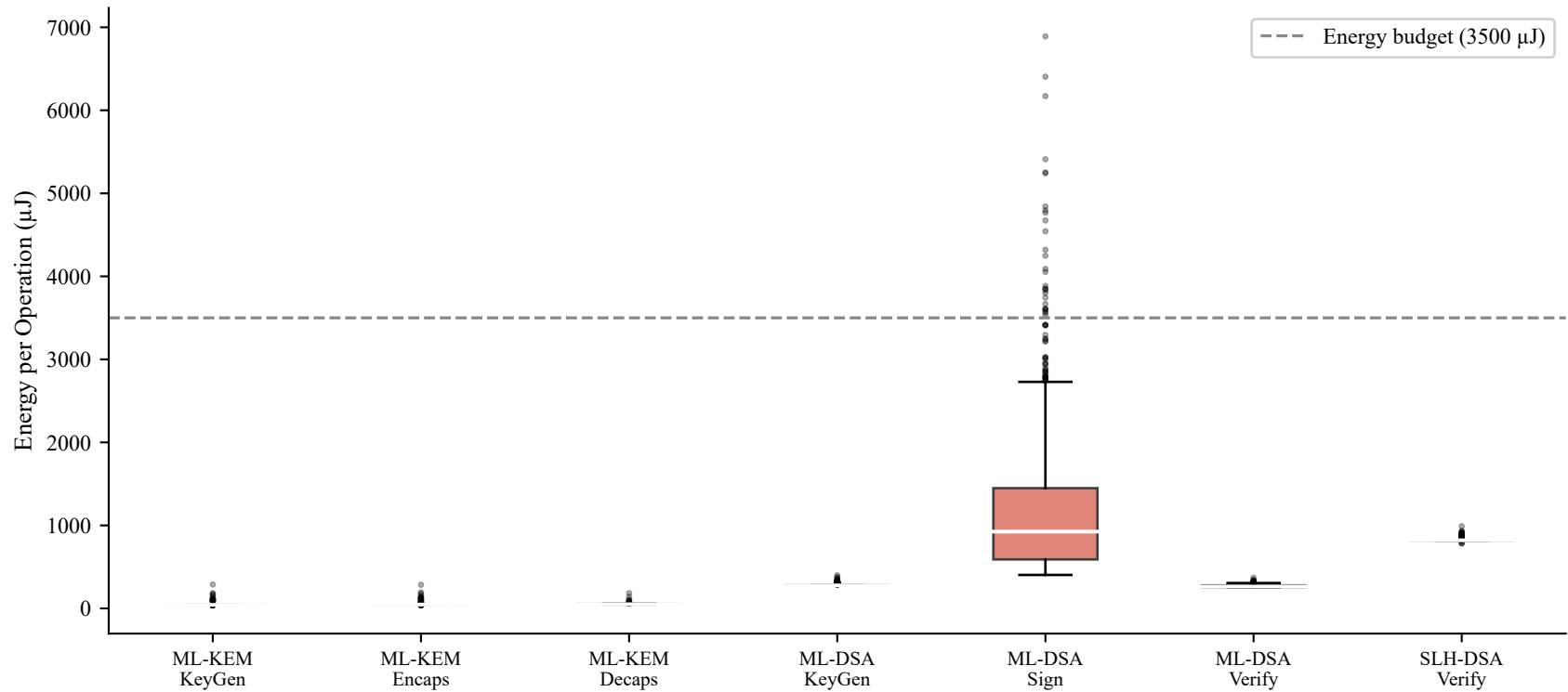
Fig. 6 Energy Distribution per Operation (Box-and-Whisker) SLH-DSA Sign excluded (883 885 \mu J median — off scale)
