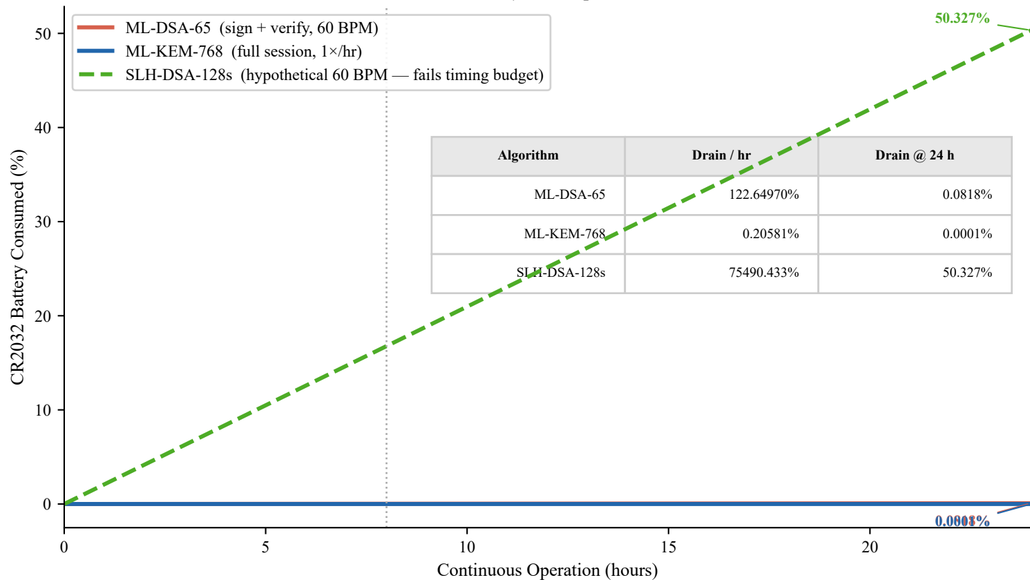
Fig. 8 Cumulative Battery Drain Projection CR2032 = 2.54 J | Active power = 14.4 mW
