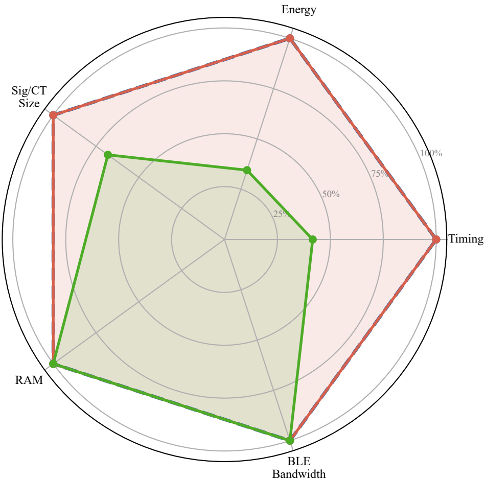
Fig. 10 Multi-Criteria Feasibility Radar Normalised scores — outer rim = fully within budget ML-KEM (dashed) scores \approx 100\% on all axes
