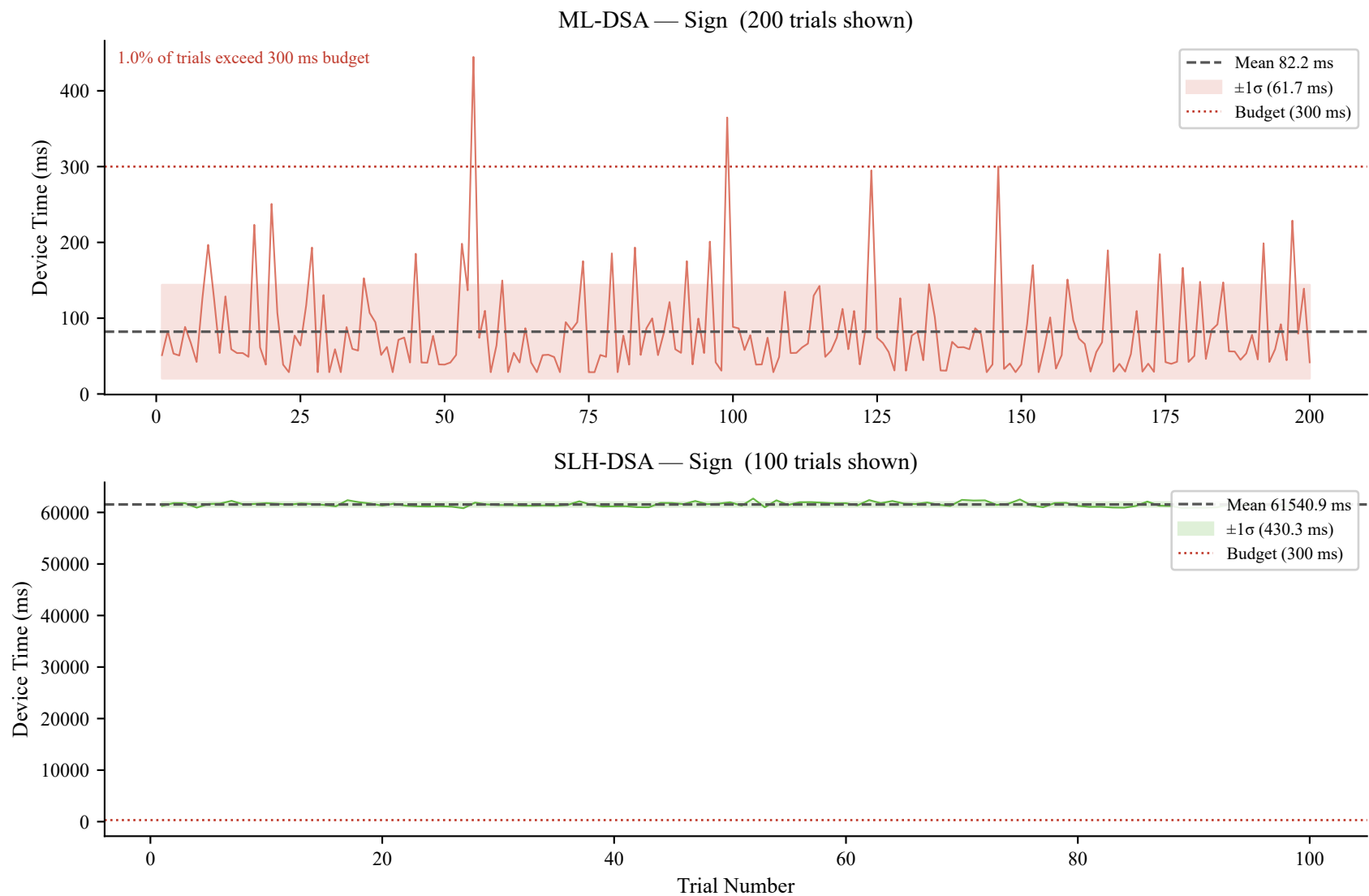
Fig. 12 Per-Trial Latency Stability — Sign Operations First 200 trials | shaded = \pm 1\sigma band
