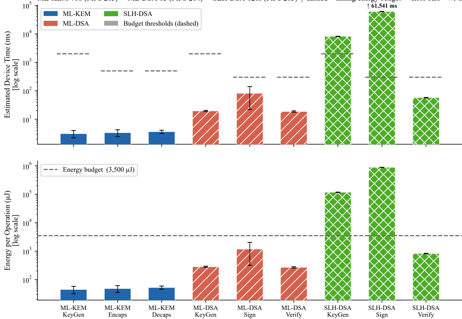
Fig. A Cryptographic Operation Performance on Nordic nRF52840 ML-KEM-768 (FIPS 203) · ML-DSA-65 (FIPS 204) · SLH-DSA-128s (FIPS 205) | dashed = timing/energy budget · error bars = \pm 1 SD
