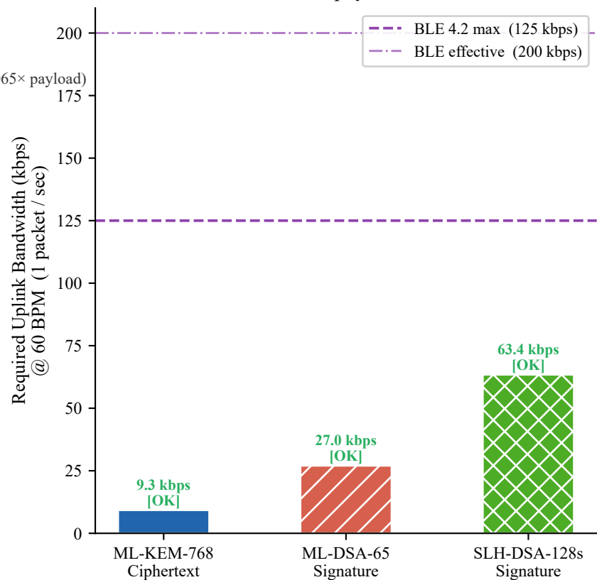
(b) Required uplink bandwidth vs BLE 4.2 physical limits
