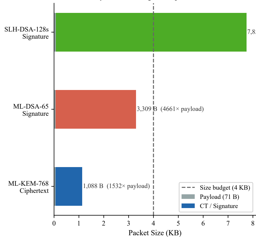
(a) Packet size breakdown Payload + CT/Signature per heartbeat
