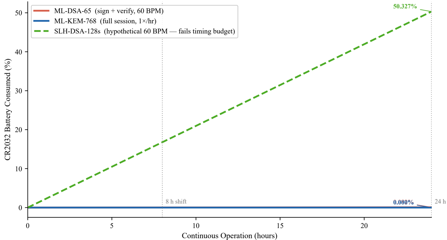
Fig. D Cumulative CR2032 Battery Drain — 24-Hour Clinical Operation CR2032 = 2.54 J · Active power model: 14.4 mW · HR = 60 BPM
