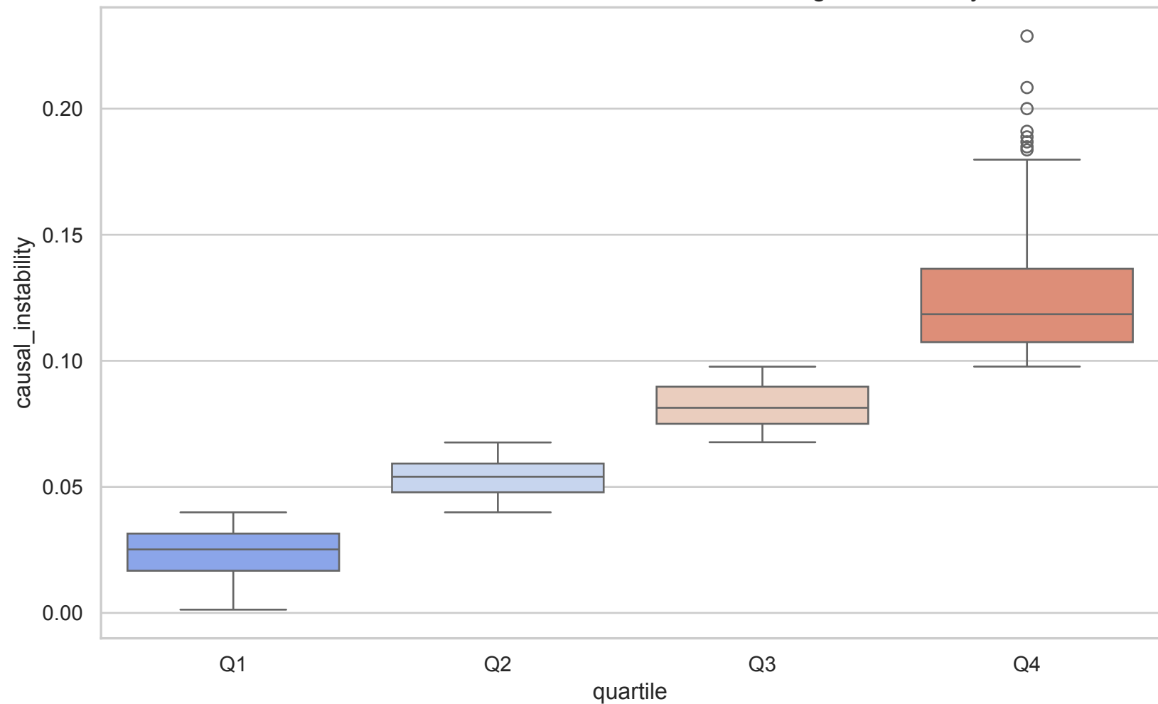
Validation: Predicted-Critical Chunks Show Higher Instability
