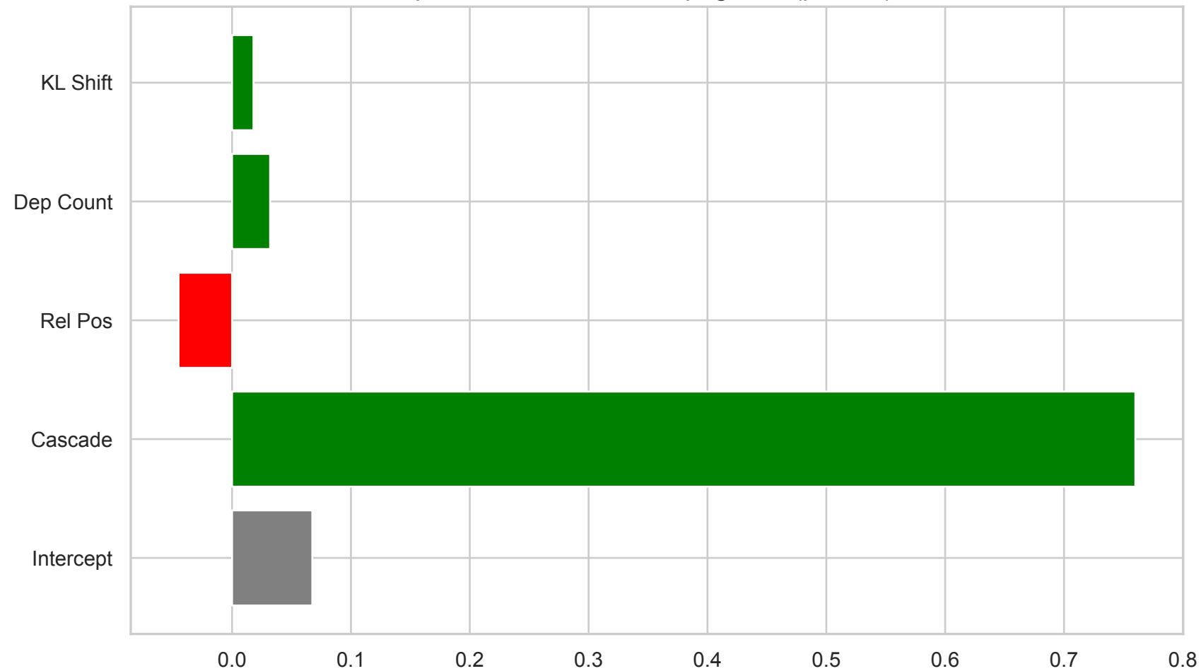
Feature Importance: Cascade Propagation ( \beta=0.76 ) Dominates
