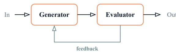
Figure 12: Workflow Evaluator–Optimizer
