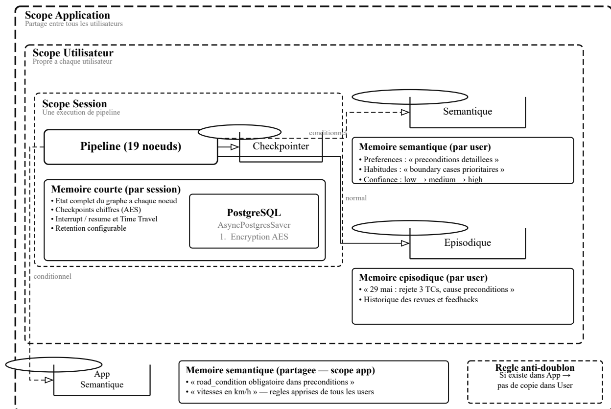
Figure 23: Architecture memoire
