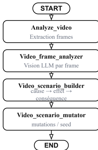
Figure 18: Agent video Workflows
