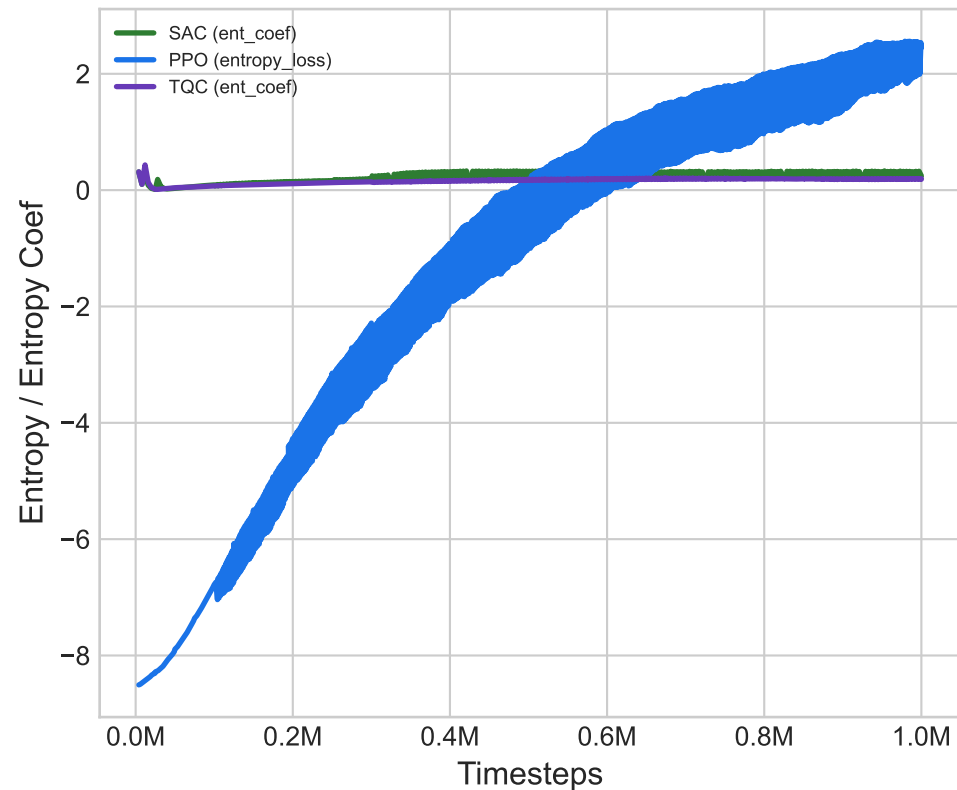
HalfCheetah
