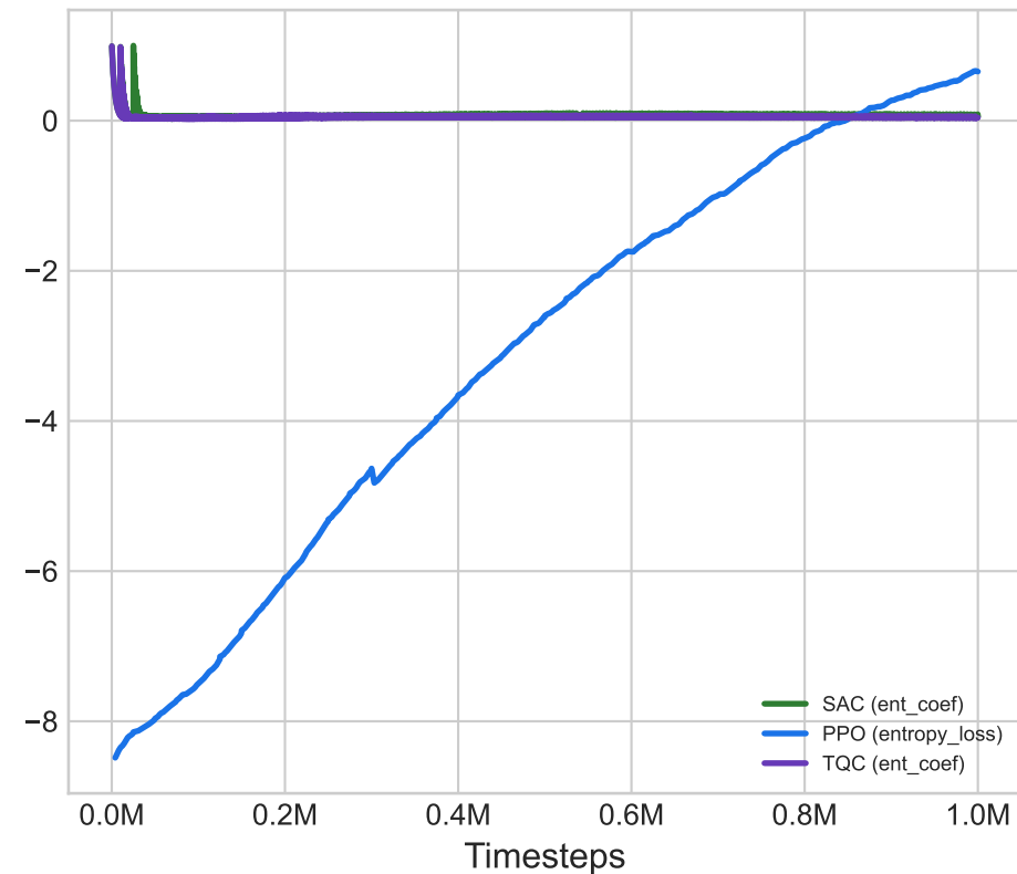
Walker2d
