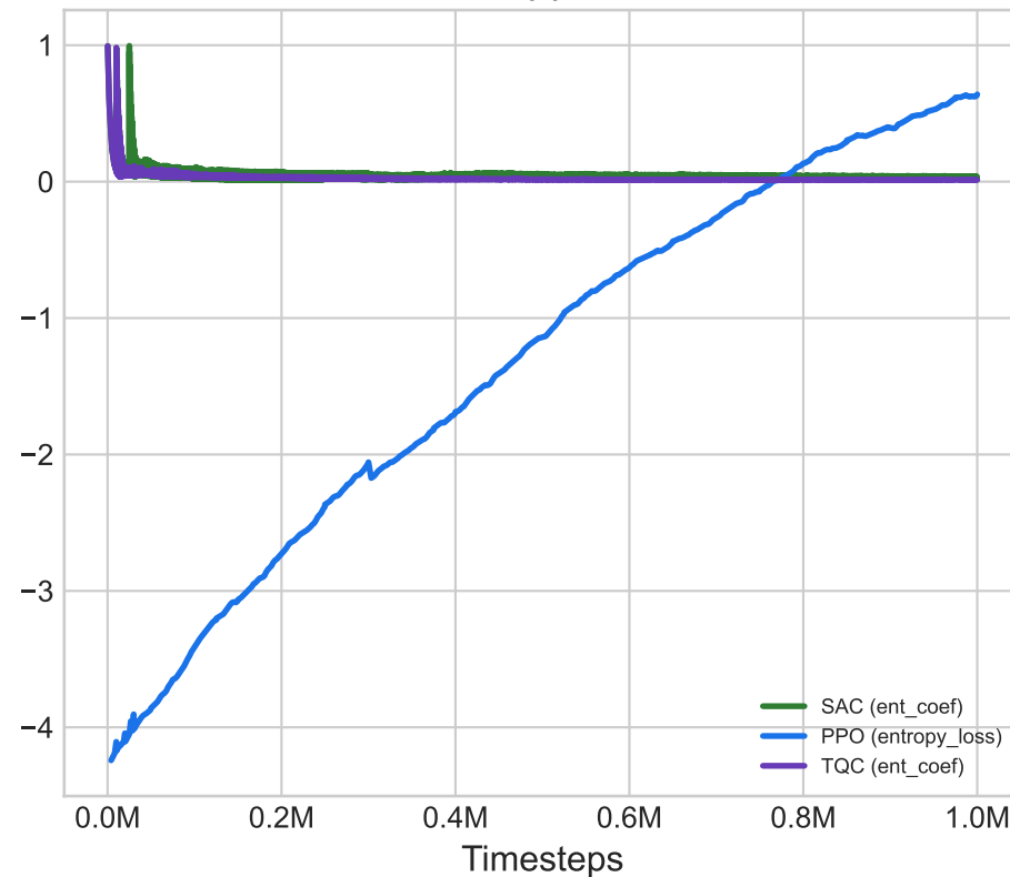
Hopper
