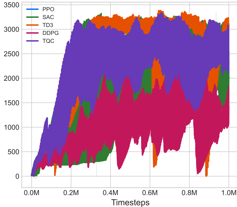
Hopper
