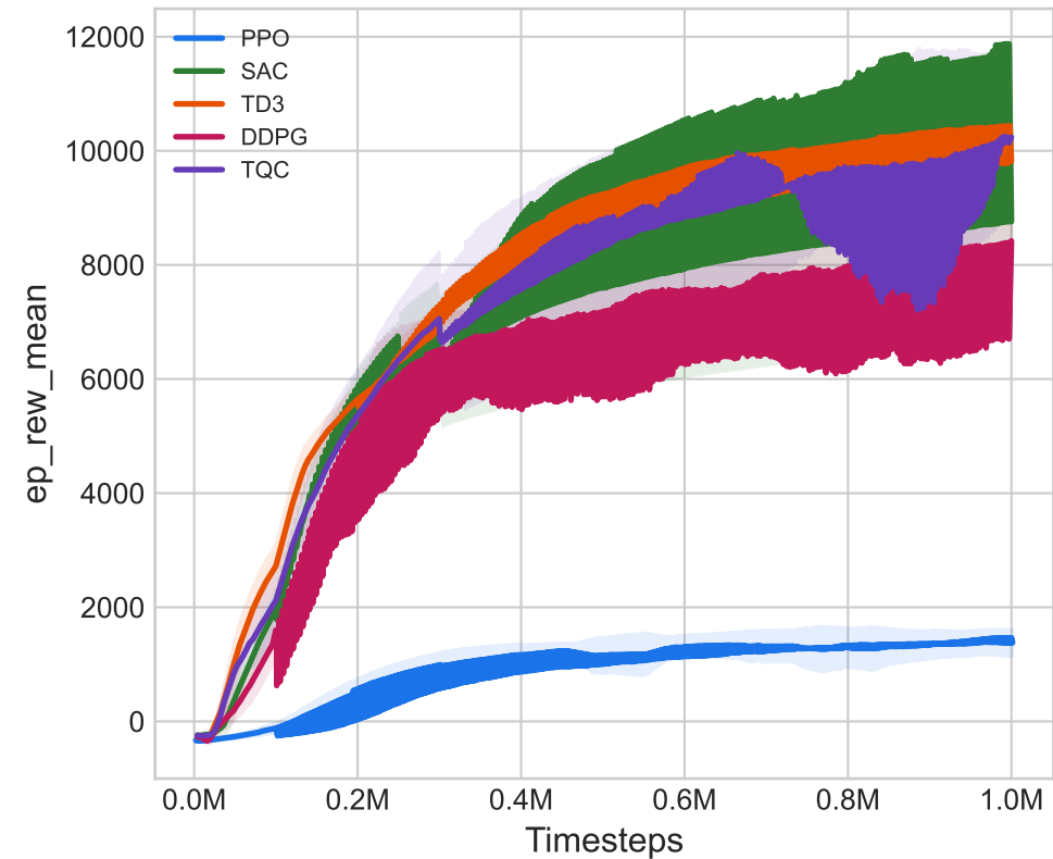
HalfCheetah
