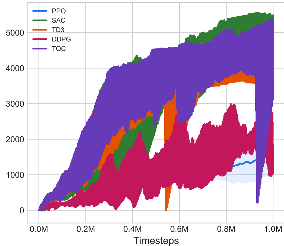
Walker2d
