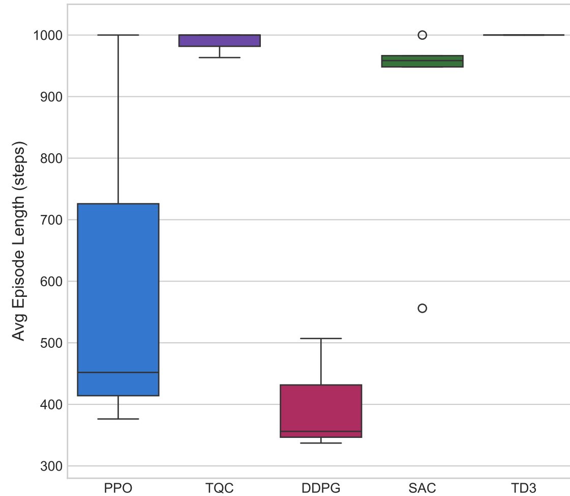
Walker2d
