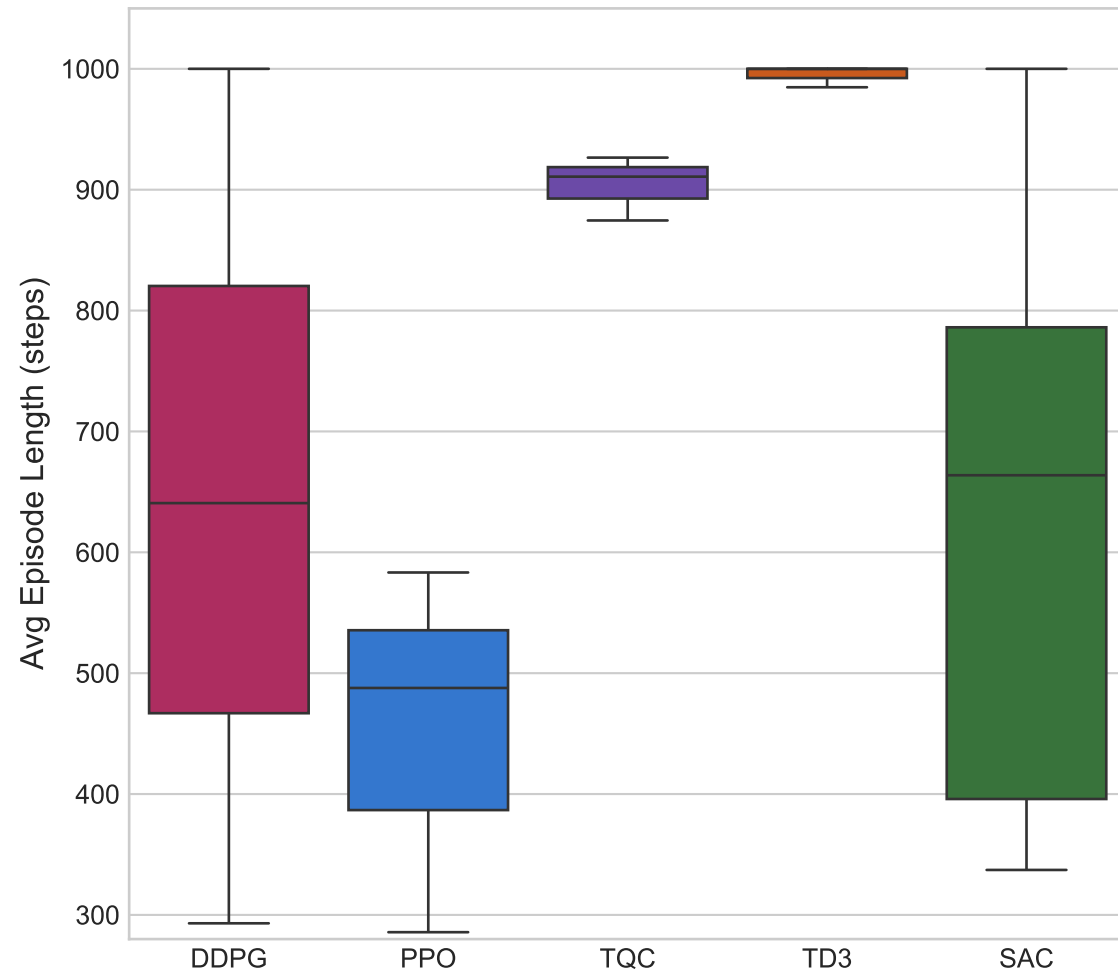
Hopper
