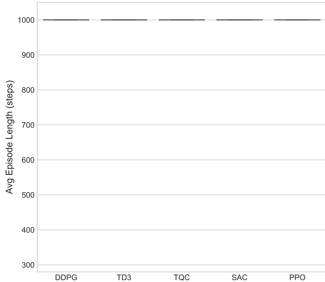
HalfCheetah
