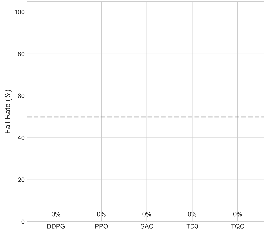
HalfCheetah
