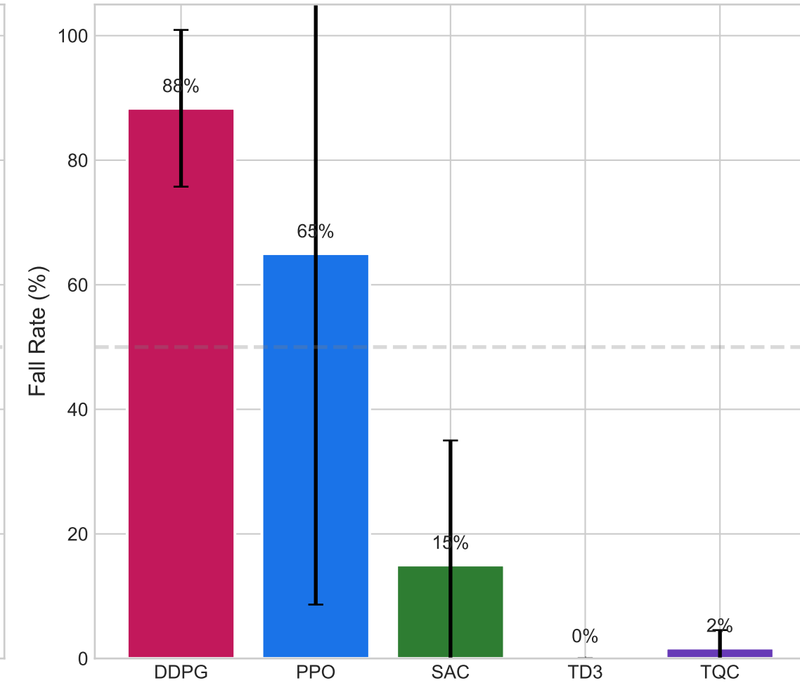
Walker2d
