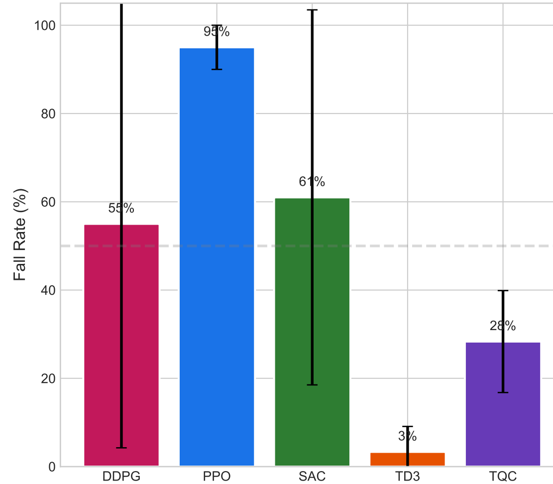
Hopper
