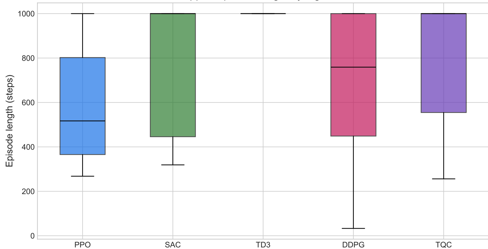
Hopper: episode length by algorithm
