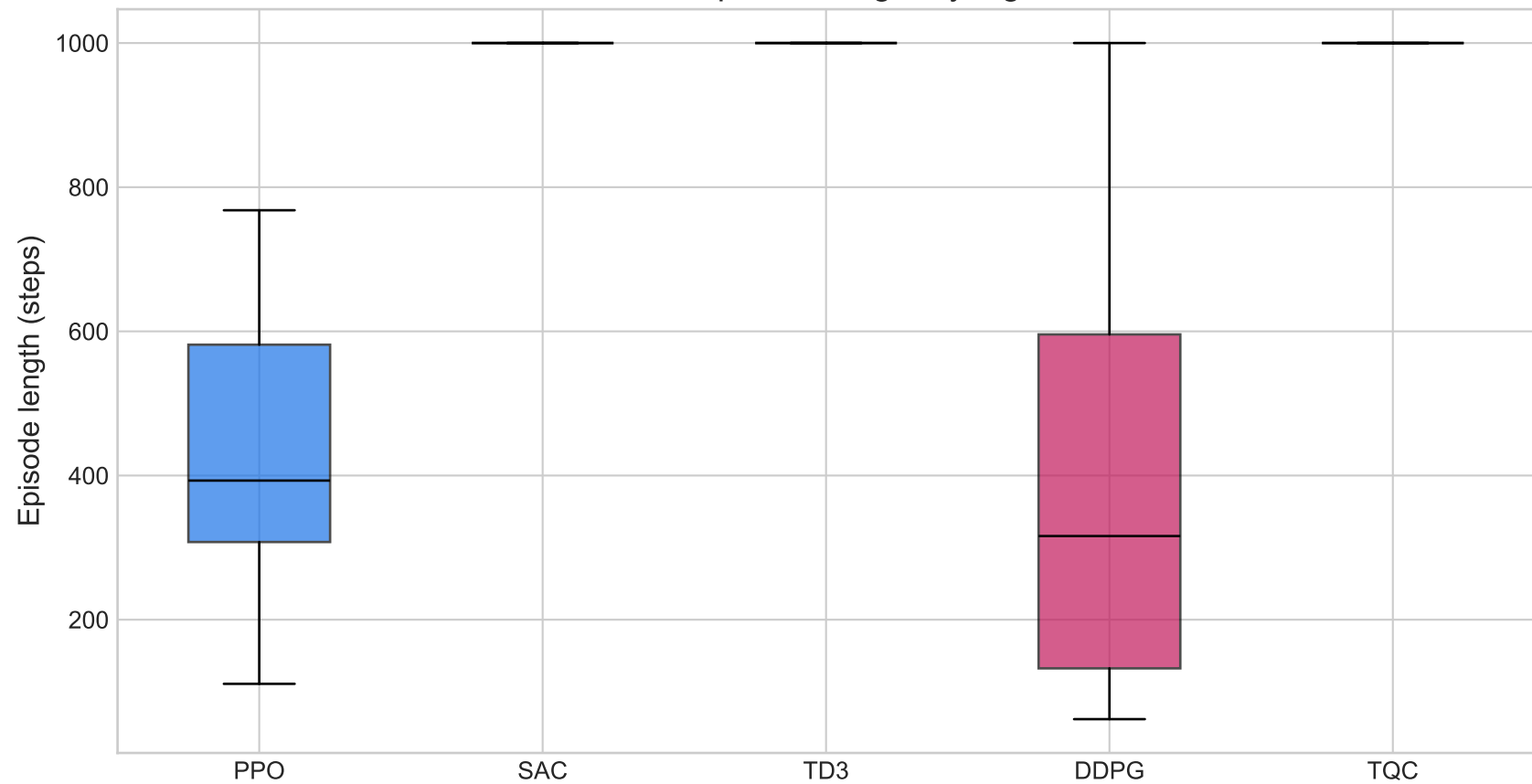
Walker2d: episode length by algorithm
