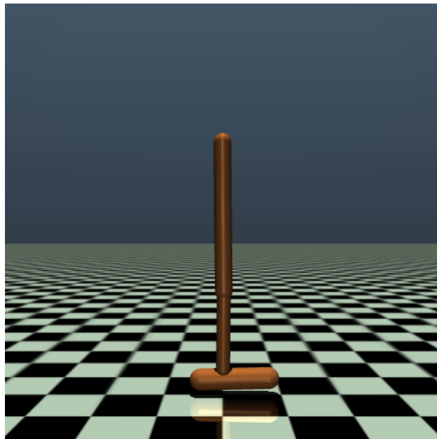
Hopper
