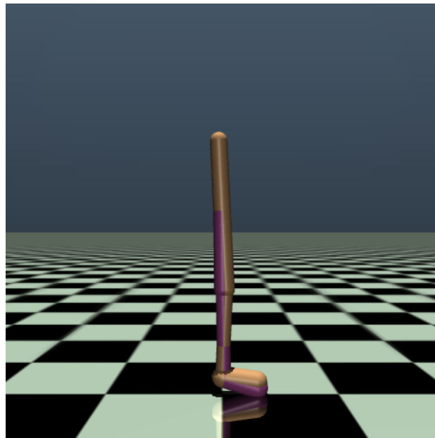
Walker2d
