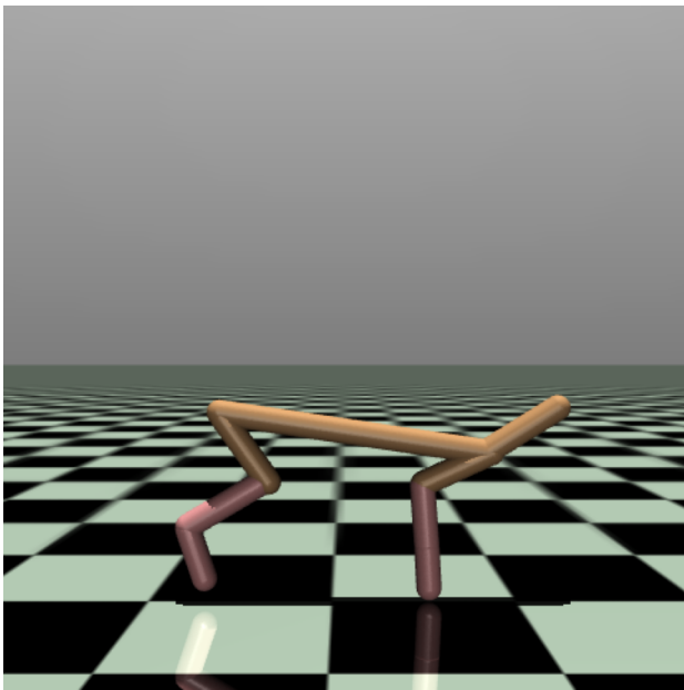
HalfCheetah
