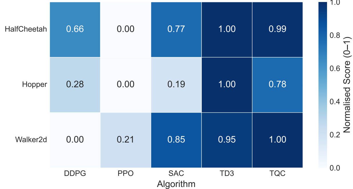
Normalised IQM Returns
