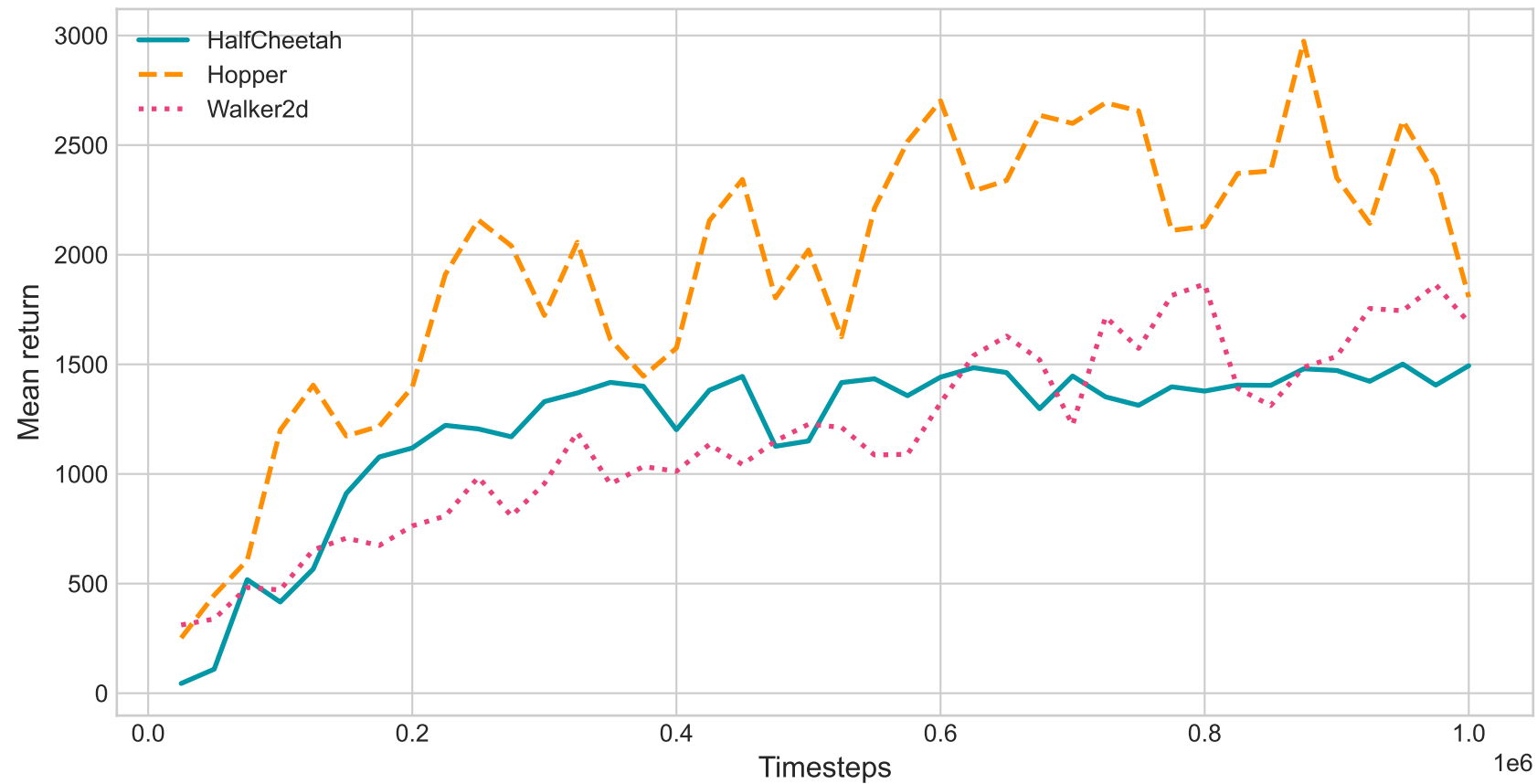
PPO across environments
