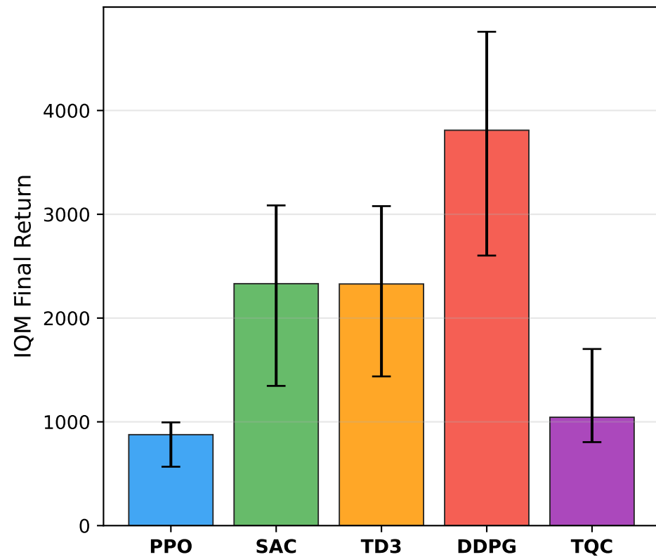
HalfCheetah-v5
