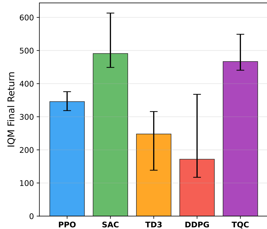
Walker2d-v5
