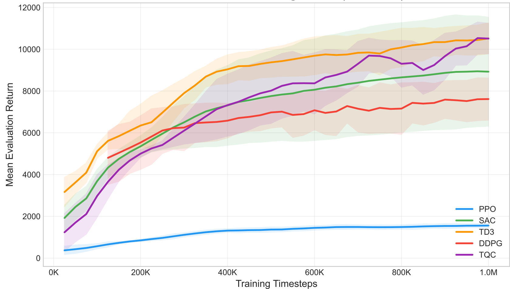
HalfCheetah-v5 — Learning Curves (Smoothed)
