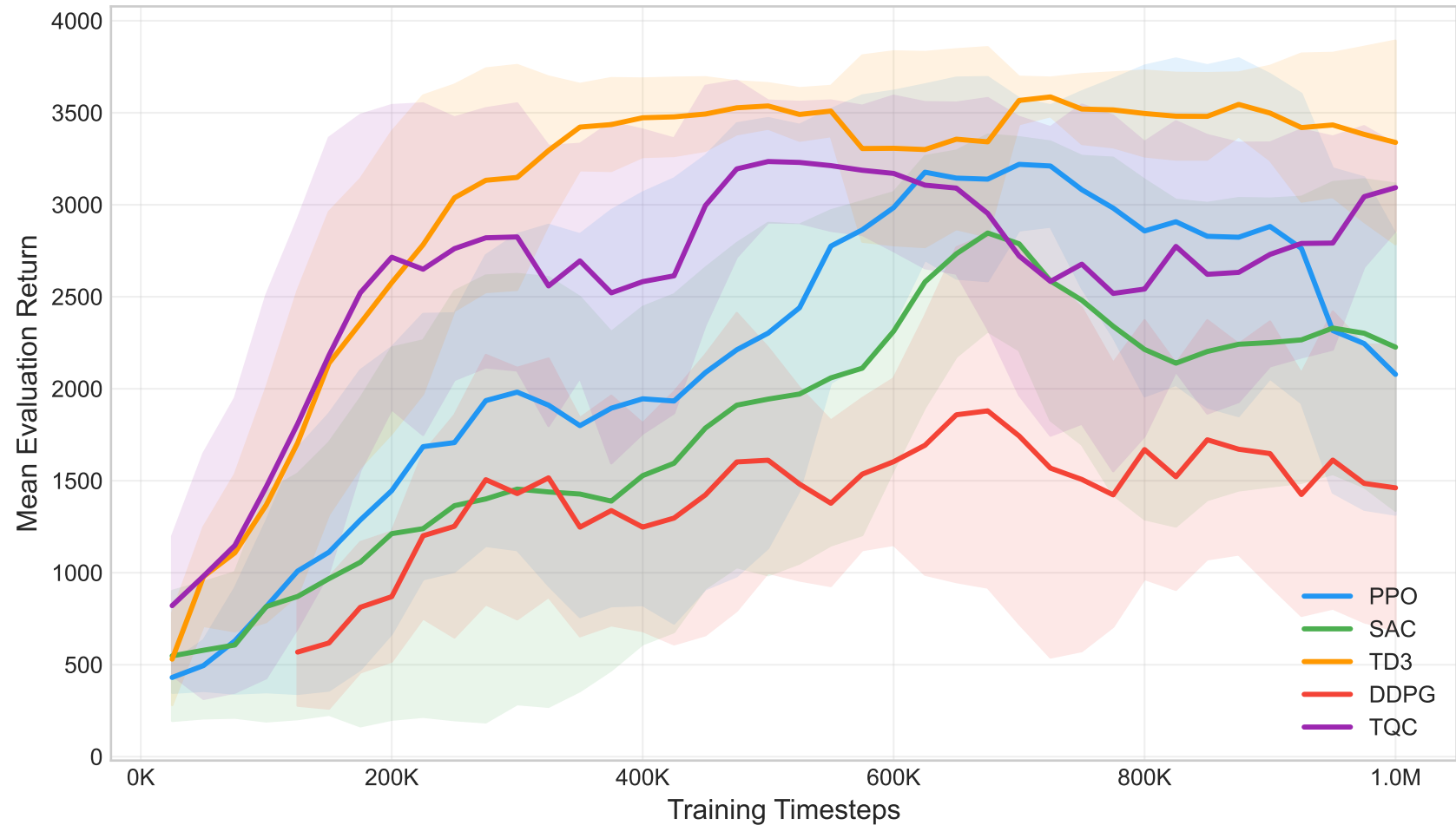
Hopper-v5 — Learning Curves (Smoothed)
