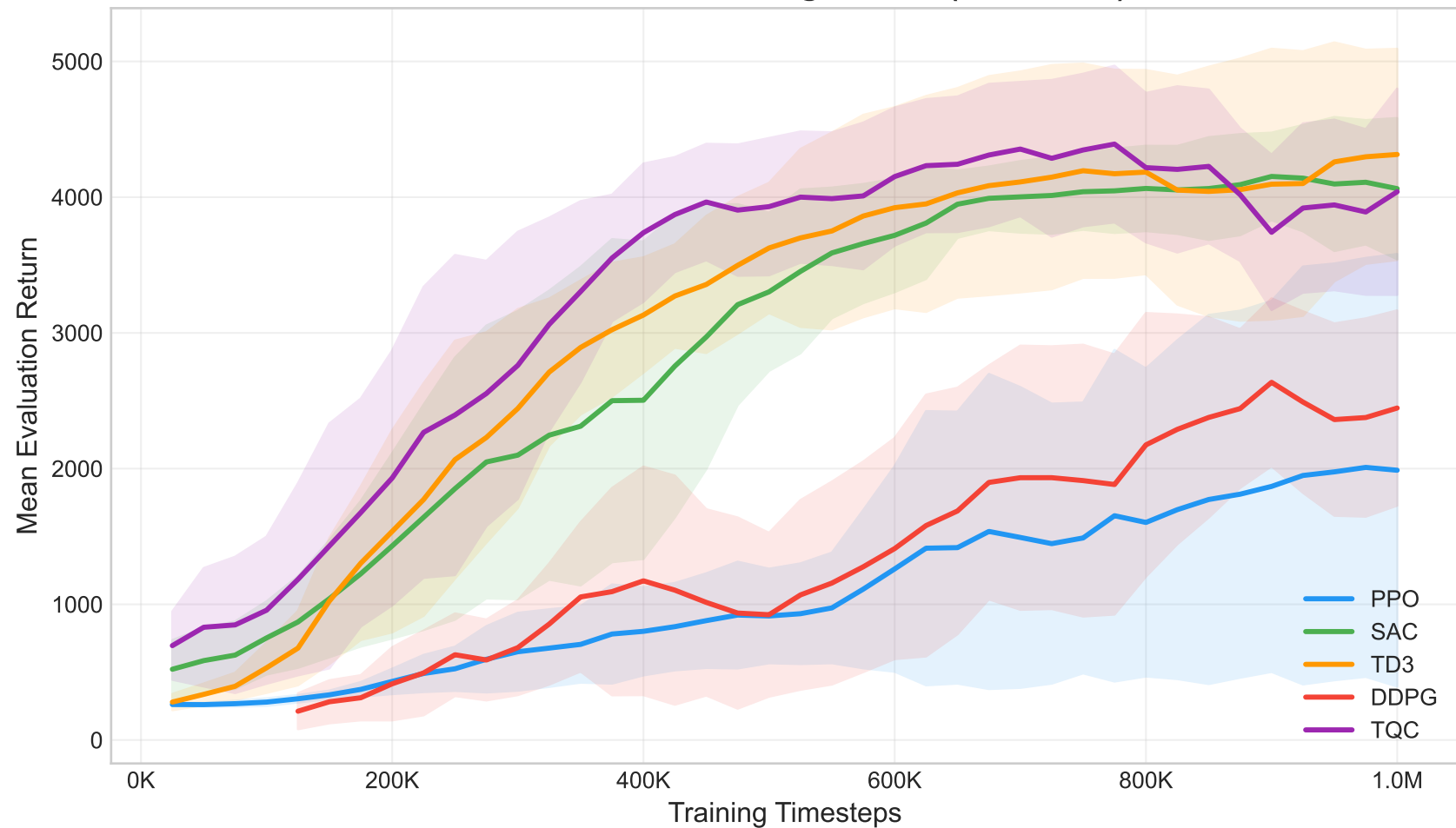
Walker2d-v5 — Learning Curves (Smoothed)
