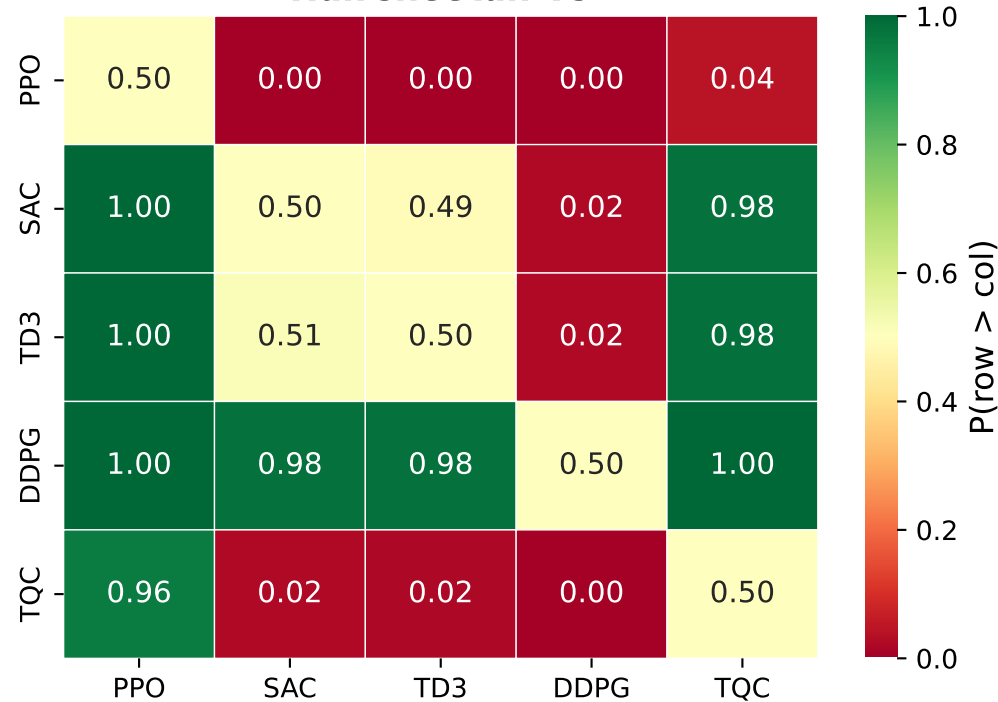
HalfCheetah-v5
