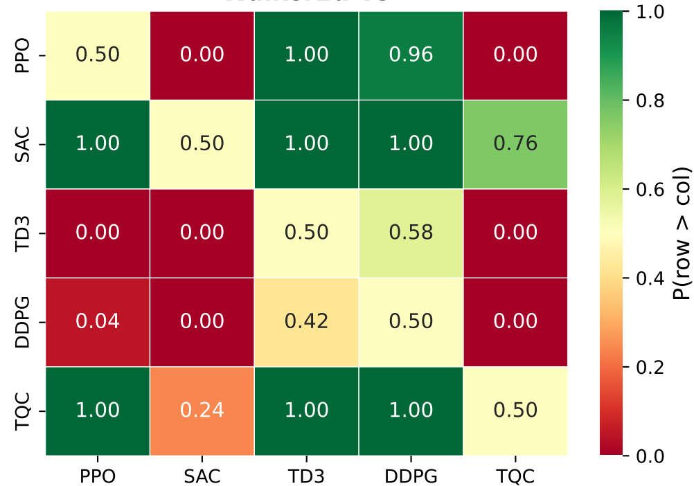
Walker2d-v5
