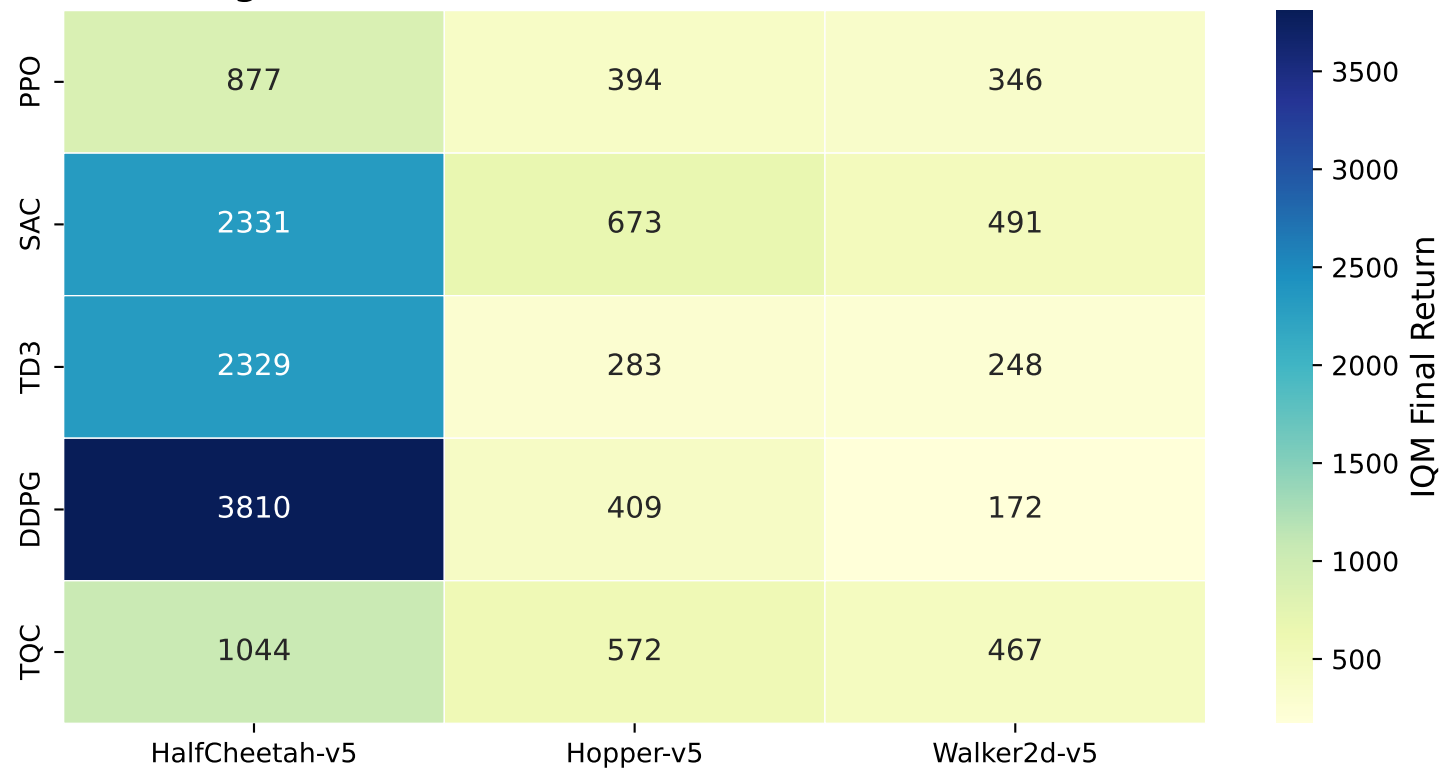
Algorithm × Environment Performance (IQM)
