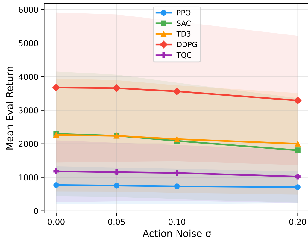
HalfCheetah-v5
