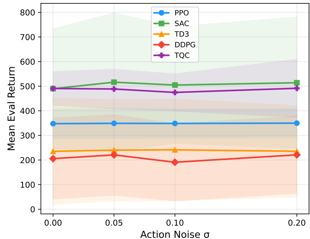
Walker2d-v5
