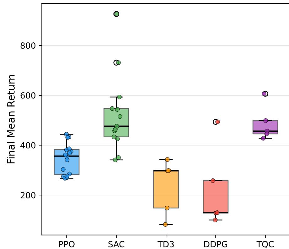
Walker2d-v5
