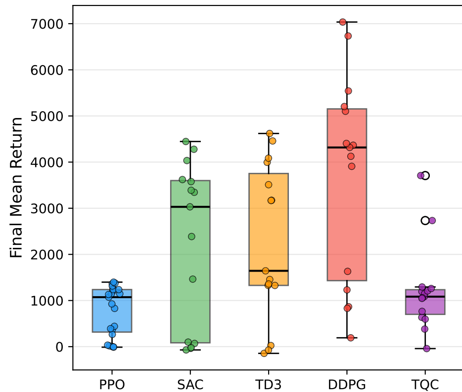
HalfCheetah-v5
