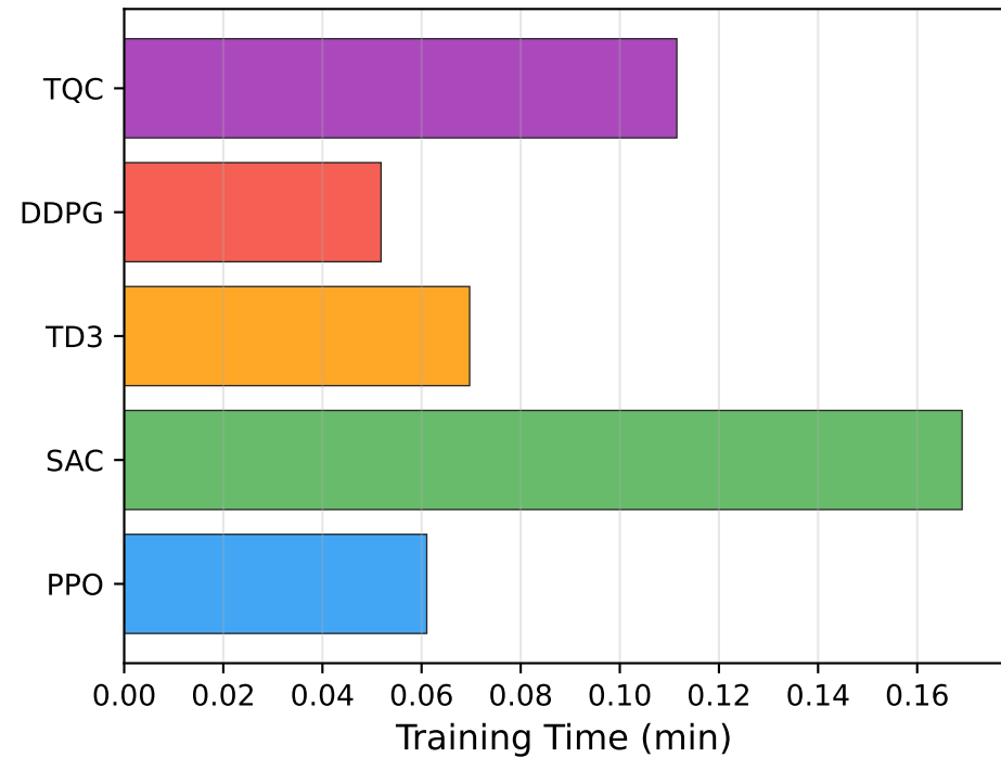
Walker2d-v5
