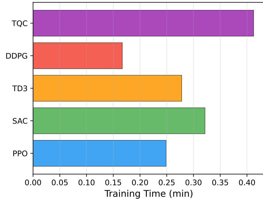
HalfCheetah-v5
