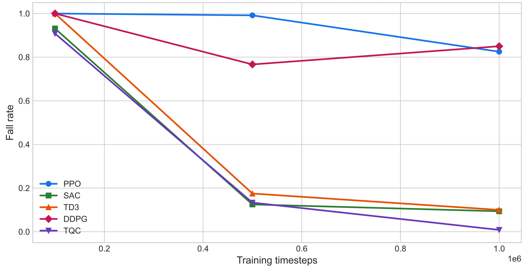
Walker2d: fall rate drops as training budget grows
