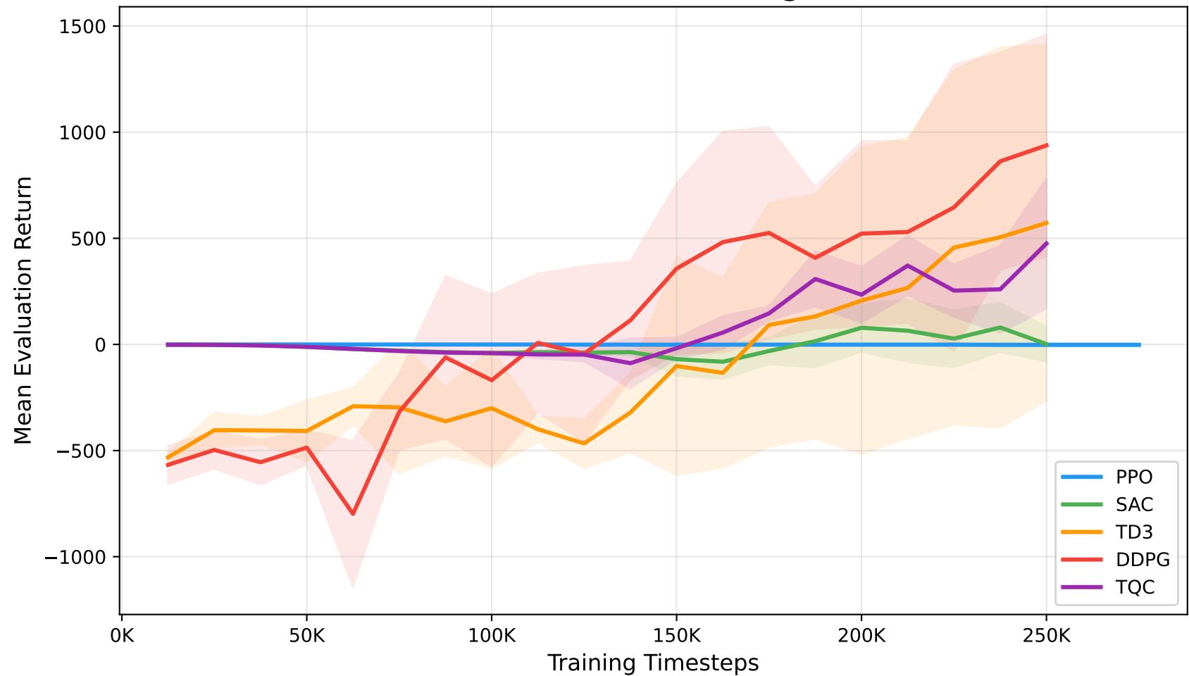
HalfCheetah-v5 — Learning Curves
