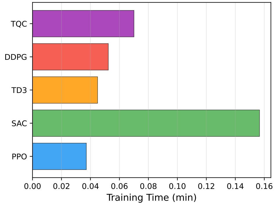
Walker2d-v5
