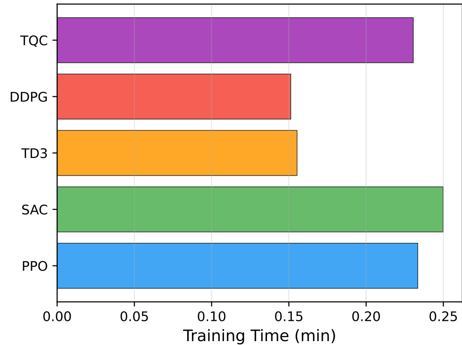
HalfCheetah-v5
